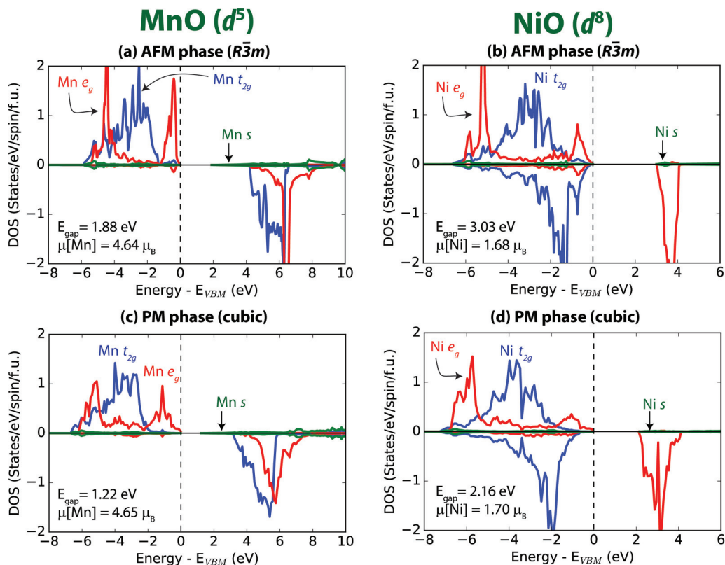
FIG. 3. Projected density of states (PDOS) on the transition metal s and d orbitals ( t_{2g} and e_g components) calculated by DFT + U ( U = 5 eV) for MnO and NiO in (a) and (b) the AFM phase with fully relaxed R\bar{3}m structures, and [(c) and (d)] the PM phase modeled by a cubic 64-atom 2 \times 2 \times 2 SQS. The lattice parameters of the SQSs are set so that the volume per formula unit is equal to the calculated volume per formula unit of the DFT + U relaxed R\bar{3}m structures of MnO and NiO.
