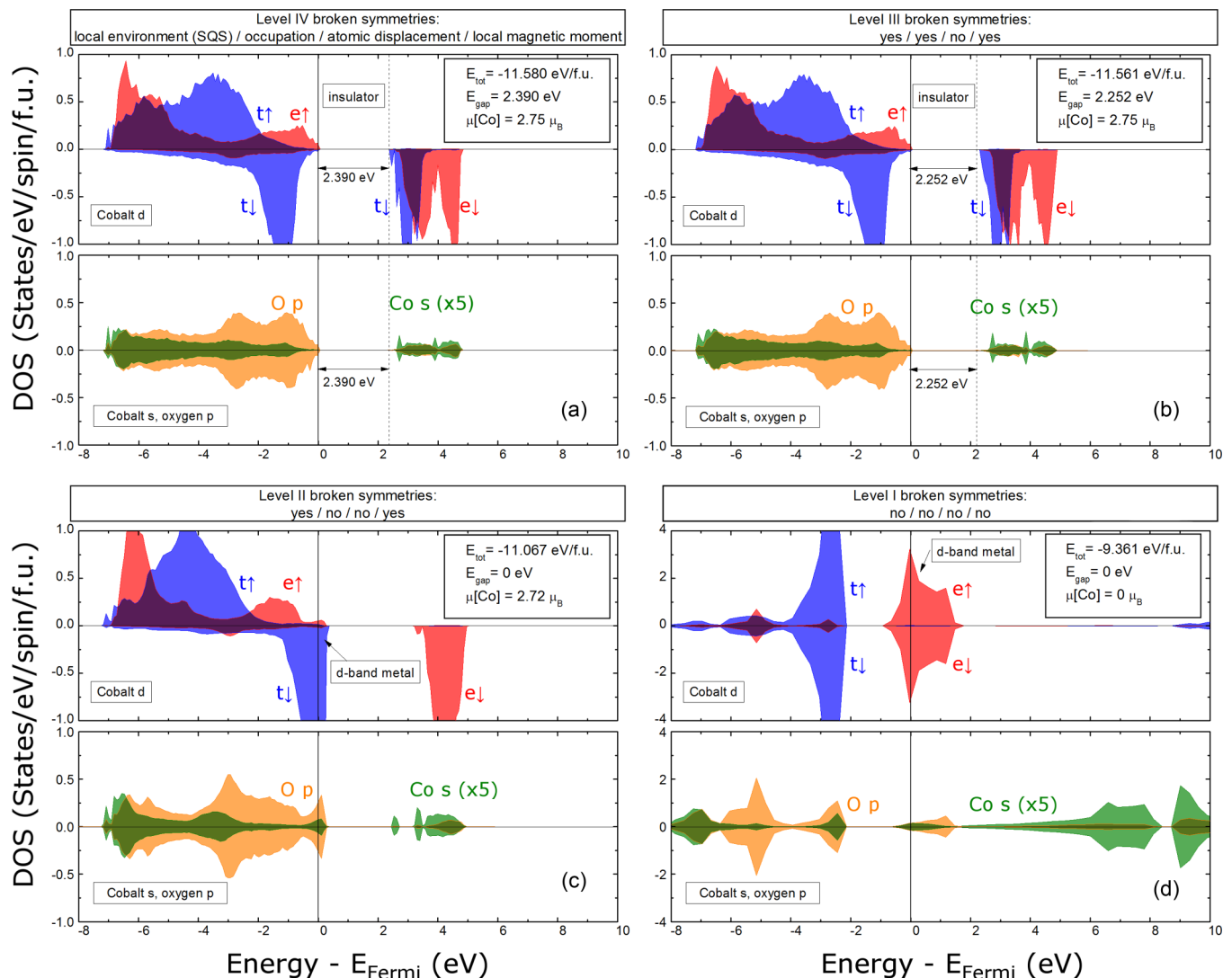
FIG. 7. Analysis of the effects of different symmetry breaking modes on the electronic structure, total energy, band gap, and local moment of paramagnetic CoO. We show the projected density of states (PDOS) on the transition-metal s and d orbitals ( t_{2g} and e_g components) and oxygen p orbitals from levels (a) IV, (b) III, (c) II, and (d) I (see Sec. VII A for definition of these symmetry breaking levels) of rock-salt CoO. (a)–(c) are calculated in a 216-atom cubic rock-salt supercell with SQS, while (d) is calculated in a two-atom rock-salt primitive cell. All lattice parameters are the same as the one used in Fig. 4(d).
