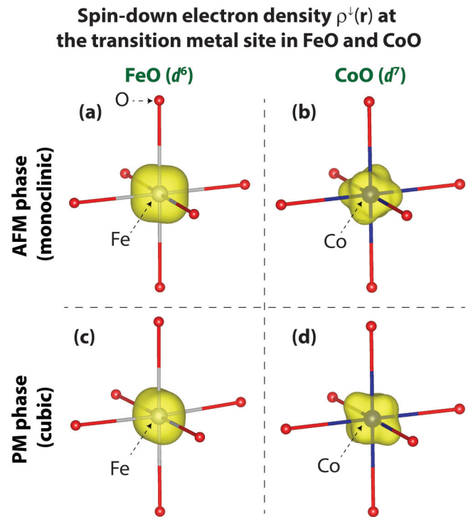
FIG. 5. (a) and (b) depict the minority-spin electron density \rho^\downarrow(\mathbf{r}) at the Fe and Co site in the AFM monoclinic phases of, respectively, FeO and CoO calculated by DFT + U . (c) and (d) depict the minority-spin electron density \rho^\downarrow(\mathbf{r}) at the Fe and Co site in the PM phase of, respectively, FeO and CoO modeled by the magnetic 64-atom cubic SQS used for the calculation of the PDOS shown in Figs. 5(c) and 5(d). The full \rho^\downarrow(\mathbf{r}) of PM FeO and CoO in the SQS is shown in Figs. 6(a) and 6(b).
