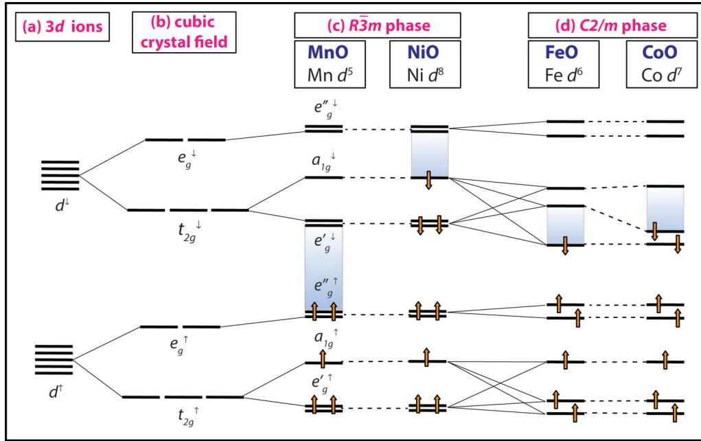
FIG. 2. Schematic of the sequence of level splittings and combinations for the d orbitals in MnO, NiO, FeO, and CoO as the exchange coupling and the crystal field of the symmetry appropriate to each phase are progressively imposed: (a) splitting of the d orbitals into the transition-metal atoms subjected to exchange coupling. (b) Splitting of the spin-up and spin-down d levels subjected to a cubic O_h crystal field: this is the case of a rock-salt structure with hypothetical Fm\bar{3}m magnetic ordering. (c) Splitting of the d level in the D_{3d} crystal field in the distorted rock-salt lattice with the rhombohedral R\bar{3}m AFM-II magnetic ordering. (d) Splitting of the d orbitals in a tetragonal crystal field as in the monoclinic C2/m phases of FeO and CoO. Note that in this schematic we emphasize the effect of the relevant interaction in progressively removing the degeneracy of the d orbitals, while we do not intend to reproduce to scale the position of the spin-up and spin-down energy levels. The reader should inspect the projected DOSs of Figs. 3 and 4 to obtain the actual calculated energy position of the d bands.
