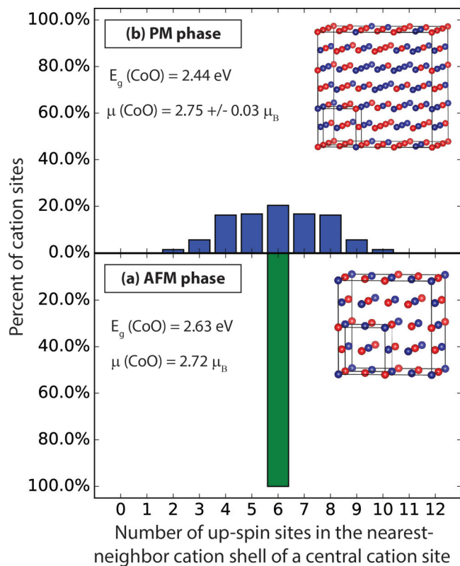
FIG. 1. Percent fraction F(n_{NN}^\uparrow) of cation sites as a function of the number n_{NN}^\uparrow of spin-up nearest-neighbor (NN) metal site of a central cation site in (a) the AFM-II phase and (b) the PM phase modeled here by the 216-atom rock-salt SQS shown in the insert (in this model only the metal sublattice of the underlying rock-salt structure is shown). In the AFM phase, n_{NN}^\uparrow = 6 for all cations, while in the PM phase, n_{NN}^\uparrow varies between 0 and 12 and F(n_{NN}^\uparrow) approximates a binomial distribution. The frequency of local environment types F(n_{NN}^\uparrow) was calculated averaging over a 216-atom SQS with A_{0.5}B_{0.5} composition and its complementary B_{0.5}A_{0.5} spin configuration. The band gap and the TM magnetic moment are reported for CoO in the AFM phase and the PM phase, which was calculated using the displayed 216-atom 3 \times 3 \times 3 SQS.
