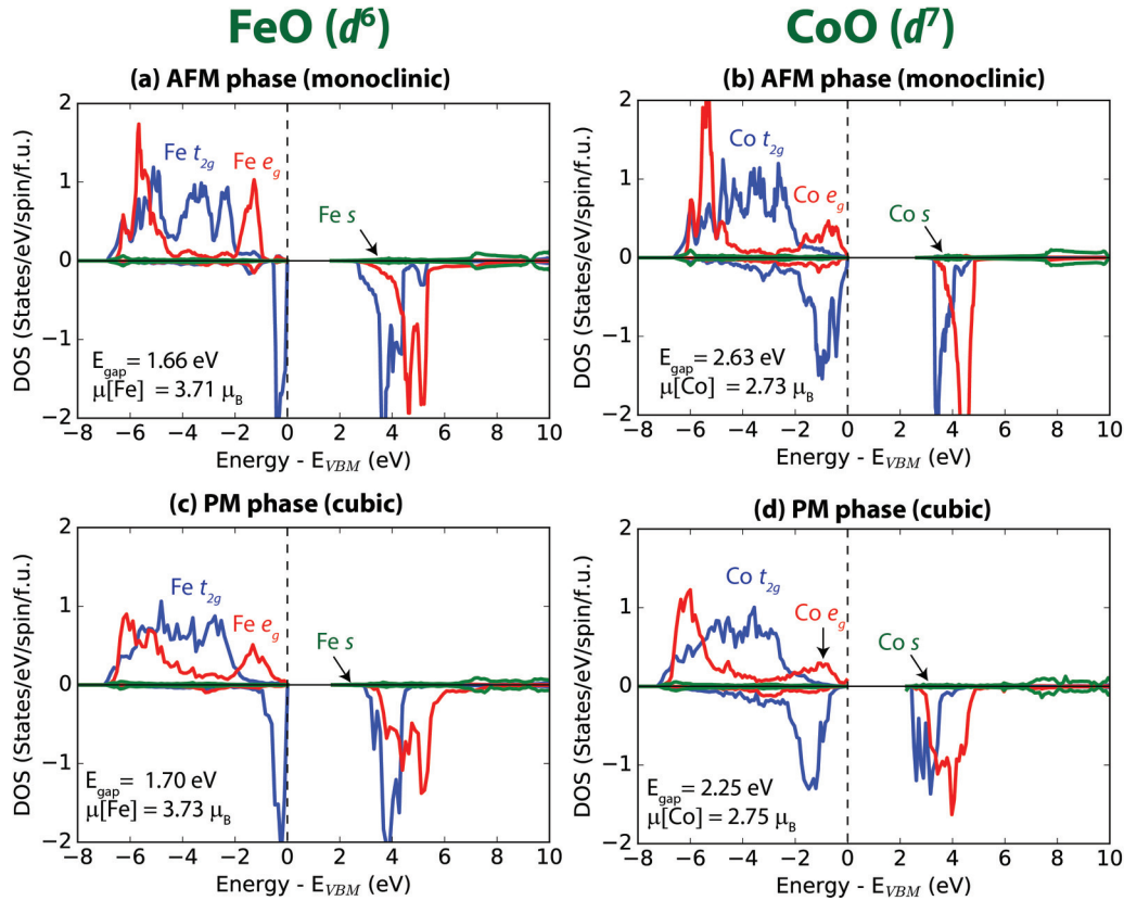
FIG. 4. Projected density of states (PDOS) on the transition metal s and d orbitals ( t_{2g} and e_g components) calculated by DFT + U ( U = 5 eV) for FeO and CoO, in (a) and (b) the AFM phases with the fully relaxed monoclinic C2/m structures, and in (c) and (d) the paramagnetic phases modeled by a cubic 64-atom 2 \times 2 \times 2 SQS. The lattice parameters of the SQSs are set so that the volume per formula unit is equal to the calculated volume per formula unit of the DFT + U relaxed C2/m structures of FeO and CoO.
