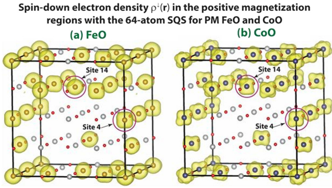
FIG. 6. Minority-spin electron density \rho^\downarrow(\mathbf{r}) in the regions with positive magnetization m(\mathbf{r}) = \rho^\uparrow(\mathbf{r}) - \rho^\downarrow(\mathbf{r}) > 0 within the magnetic 64-atom SQS cell used in the DFT + U ( U = 5 eV) calculations of the PM phases of (a) FeO and (b) CoO. To avoid visual clutter, we masked out the regions of space within spheres of radius centered at the oxygen sites.
