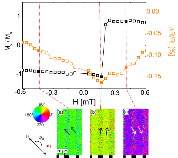
FIG. 4. y component of M (along stripe length) (black squares) and relative resistance change (orange squares) as a function of applied field for a sample with w = 15 \mu\text{m} | 20 \mu\text{m} (implanted | nonimplanted) stripes at \varphi_H = 135^\circ . R_s is the resistance of the sample measured at magnetic saturation in \varphi_H = 135^\circ direction. The field (current) direction is denoted by black (dashed red) arrows. (a)–(c) Corresponding domain images taken at field values marked with dotted lines in the upper panel. The color code denotes the magnetization direction. Black (white) rectangles mark implanted (nonimplanted) stripes. Only one field sweep direction (from negative to positive field) value is shown for the images.
