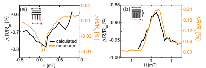
FIG. 8. Comparison of directly measured AMR and AMR calculated from Kerr images for composite stripe structures of series 4 with (a) w = 8 \mu\text{m} stripes and \varphi_H = 0^\circ and (b) w = 2 \mu\text{m} stripes and \varphi_H = 90^\circ .
