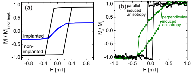
FIG. 1. (a) VSM measurements with the field applied parallel to the induced anisotropy axis for the nonimplanted film (black curve) and implanted film (blue curve). (b) Magnetization with external field applied parallel to the induced anisotropy (black curve) and perpendicular to it (green curve).
