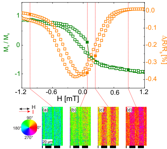
FIG. 3. x component of M perpendicular to the main stripe axes (green squares) and relative resistance change (orange squares) as a function of applied field sample with w = 20 \mu\text{m} | 15 \mu\text{m} (implanted | nonimplanted) stripes at \varphi_H = 0^\circ . The field (current) direction is denoted by a black (dashed red) arrow. (a)–(c) Corresponding domain images taken at field values marked with dotted lines in the upper panel. The color code denotes the magnetization direction. Black (white) rectangles mark implanted (nonimplanted) stripes. Note that only one field sweep direction (from negative to positive field) value is shown for the images.
