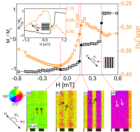
FIG. 5. y component of M (along stripe length) (black squares) and relative resistance change (orange squares) as a function of the applied field for sample with w = 20 \mu\text{m} | 15 \mu\text{m} (implanted| nonimplanted) stripes at \varphi_H = 135^\circ . The field (current) direction is denoted by a black (dashed red) arrow. (a)–(d) Corresponding domain images taken at field values marked by dotted lines in the upper panel. Black (white) rectangles mark implanted (nonimplanted) stripes. Only one field sweep direction from negative to positive field values is shown. The inset shows the measurements of the M component the along stripe length (black line) and relative resistance change (orange line) when the current is applied parallel to the stripe axis. R_s is the resistance of the sample measured at saturation for the chosen field direction.
