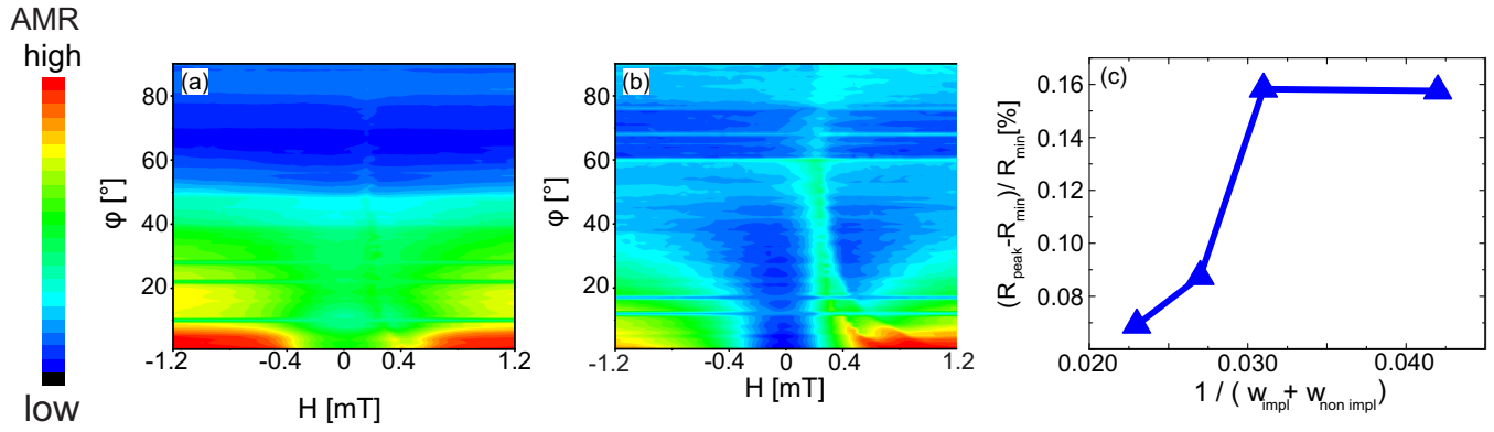
FIG. 6. Measurement of the AMR at different field angles \varphi for (a) a permalloy film and (b) a stripe sample with w = 16 \mu\text{m} | 16 \mu\text{m} (implanted| nonimplanted) stripes. (c) Dependence of the height of the extra peak at the interface on the sum of implanted and nonimplanted stripe width ( w_{\text{impl}} + w_{\text{nonimpl}} ).
