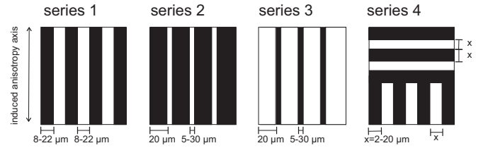
FIG. 2. Sketch of the four different sample layouts. The stripe width is given in \mu\text{m} . Black (white) color represents implanted (nonimplanted) stripes. The double headed arrow denotes the induced anisotropy axis.
