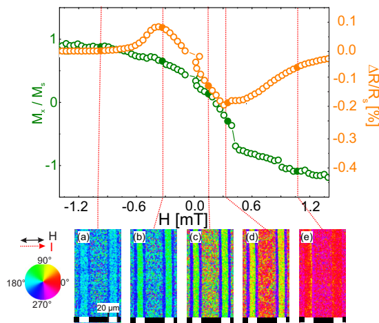
FIG. 7. AMR measurements on sample with w = 30 \mu\text{m} | 20 \mu\text{m} (implanted| nonimplanted) stripes and \varphi_H = 0^\circ . R_s is the resistance of the sample measured at magnetic saturation in \varphi_H = 0^\circ direction.
