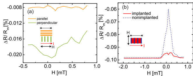
FIG. 9. Comparison of calculated AMR composite stripe structures (series 4). (a) Influence of stripe orientation for w = 8 \mu\text{m} and \varphi_H = 0^\circ and (b) influence of implantation for w = 2 \mu\text{m} and \varphi_H = 0^\circ .
