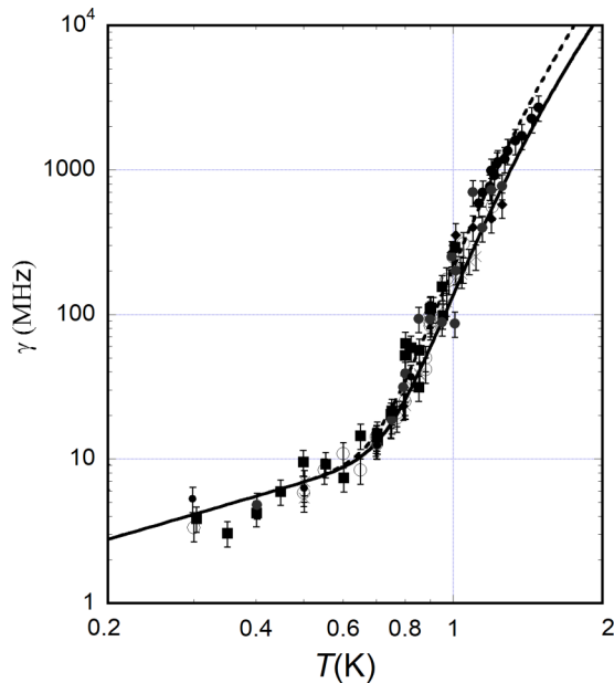
FIG. 5. Temperature-dependent contribution to the Lorentzian linewidth \gamma(T) versus temperature at 189.6 GHz. Measurements of the line-shape height and width (■, ●) were used to obtain \Delta\gamma(T) = \gamma(T) - \gamma(0.3) , relative to the value at 0.3 K. Data from Grimes et al. [2], scaled for the different pressing field, are shown (○). The solid line is the theory by Ando [13], while the dashed line shows Ando's theory with the vapor-atom scattering contribution scaled by a factor of 1.6.
