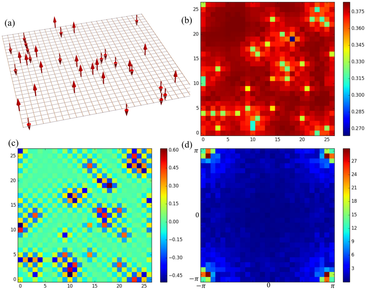
FIG. 3. Configurations of (a) impurity spins, (b) amplitude of the d -wave order parameter, (c) droplets of SDW, and (d) spin structure factor obtained after averaging over random distribution of impurities. Here \mu_S = 8t_1 , H_x = 0 , and T = 0.01t_1 .
