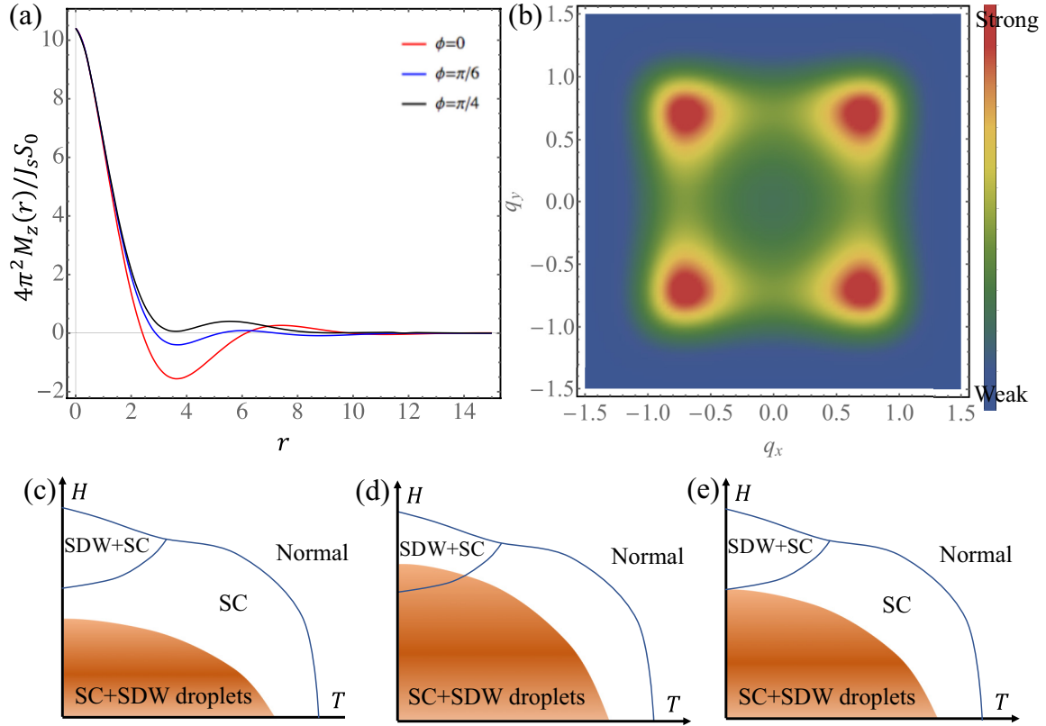
FIG. 1. (a) Magnetization profile for different angle \phi between \mathbf{r} and the x axis according to Eq. (3). (b) Impurity-induced spin structure factor. Here \gamma = \eta = 1/2 and \alpha = 1 . (c)–(e) Schematic view of the phase diagram for d -wave superconductor (SC) at the brink of SDW instability doped by dilute magnetic impurities. In the shaded region, droplets of local SDW are induced by impurities.
