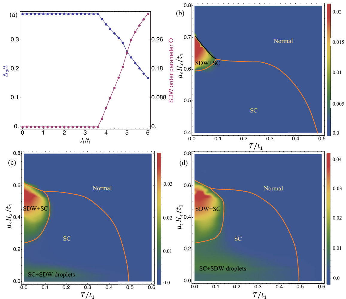
FIG. 2. (a) SDW and d -wave order parameter as a function of J_1 at zero temperature. Temperature-magnetic field phase diagram for (b) clean system, (c) system with impurities with \mu_s/t_1 = 8 (lower saturation field), and (d) system with impurities with \mu_s/t_1 = 5 (higher saturation field). Orange (black) lines denote the second (first)-order phase transition. The impurity concentration is 5%. The magnetization induced by impurities in the normal state has been subtracted.
