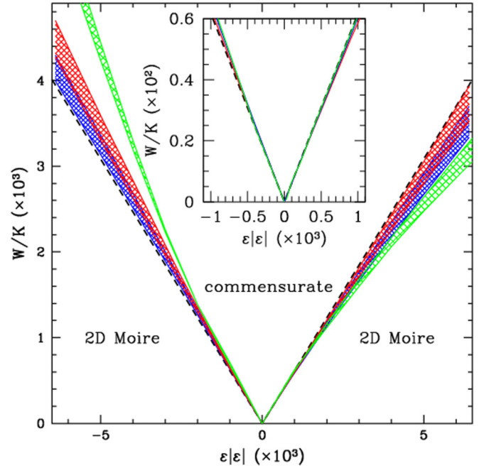
FIG. 9. Phase diagram for TH (\sqrt{3} \times \sqrt{3})R30^\circ ordering using the full PFC model with n^2 V coupling (green), the APFC model with n^2 V (red) and n^3 V (blue) coupling. The black dashed lines correspond to the sine-Gordon solution for the stripe-commensurate transition. In each case in the hatched region the stripe state is the lowest energy state and below (above) this region the 2DM (commensurate) state is the lowest energy state. The n^2 V result is redrawn from Ref. [47].
