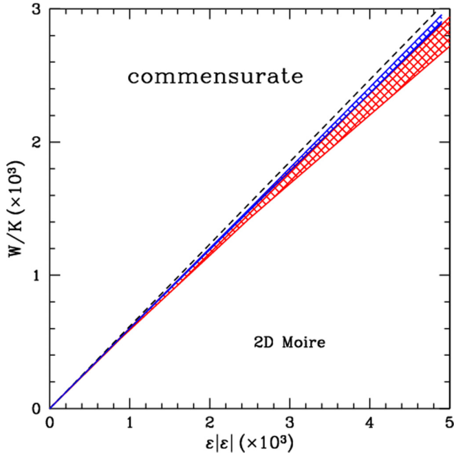
FIG. 13. Phase diagram for the (2 \times 2) and (\sqrt{7} \times \sqrt{7})R19.1^\circ systems in blue and red, respectively. The hatched regions correspond to parameter ranges where the stripe phase is the ground state.
