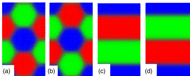
FIG. 10. Sample 2D moiré (a and b), and stripe (c and d), patterns for \epsilon = -3\% (a and c) and \epsilon = +3\% (b and d), obtained from the n^3V coupling in the TH ( \sqrt{3} \times \sqrt{3} )R30° system. In (a) (W/K, L_x, L_y) = (-0.05432 \times 10^{-2}, 364.0, 630.5) , (b) (W/K, L_x, L_y) = (-0.05160 \times 10^{-2}, 380.0, 658.2) , (c) (W/K, L_y) = (-0.05786 \times 10^{-2}, 584.0) , and (d) (W/K, L_y) = (-0.05378 \times 10^{-2}, 588.0) .
