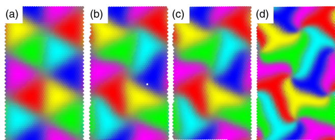
FIG. 20. Series of configurations for the TT (\sqrt{7} \times \sqrt{7})R19.1^\circ system showing colored density maxima plots of the 2D twisted moiré state. In panel (a) the honeycomb state is at (V_0, \varepsilon, L_x) = (0.00076, 3\%, 130) , and the twisted honeycomb states in (b)–(d) correspond to (V_0, \varepsilon, L_x) = (0.00078, 3\%, 132) , (0.00081, 3\%, 138) , and (0.00150, 3\%, 170) .
