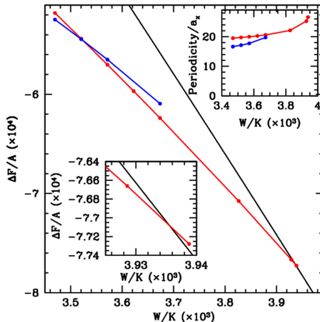
FIG. 12. Free-energy density difference from an incommensurate ( W/K = 0 ) state as a function of W/K for 2D moiré (blue), striped (red), and commensurate (black) phases at \epsilon = 8\% . In the bottom left inset is a blowup showing that the free energy of the stripes becomes higher than that of the commensurate phase indicating a discontinuous phase transition. In the top inset the periodicity of the 2D moiré (blue) and striped (red) states is shown.
