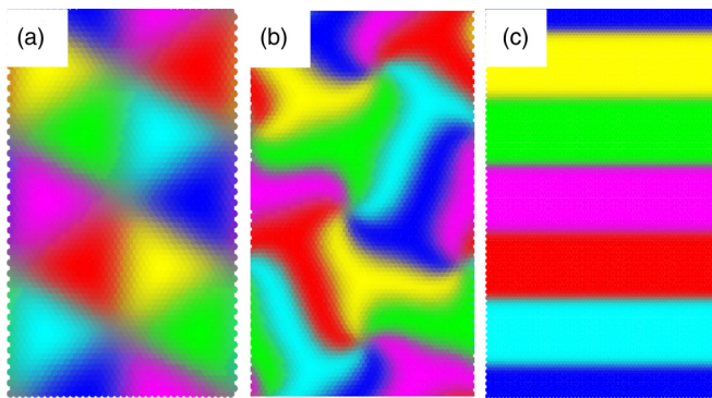
FIG. 17. Sample configurations for the TT (\sqrt{3} \times \sqrt{3})R30^\circ system showing 2D moiré, twisted 2D moiré, and striped states in (a), (b), and (c), respectively, at \varepsilon = 3\% . Here W/K = 0.574 \times 10^{-3} , 0.112 \times 10^{-3} , and 0.574 \times 10^{-3} in (a), (b), and (c), respectively.
