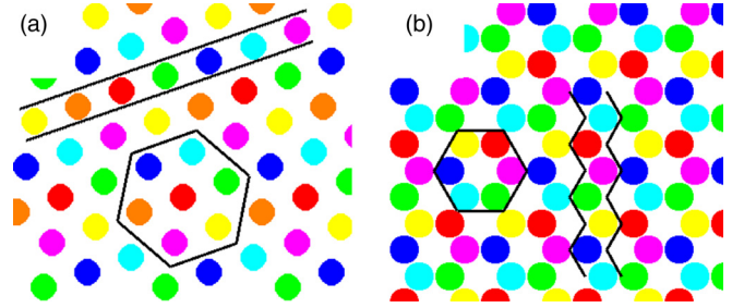
FIG. 7. In (a) the seven commensurate sublattices are shown in different colors for a (j,m) = (2,1) TH system. In (b) the six commensurate sublattices are shown for a (j,m) = (1,1) TT system. In both cases the parallel (or jagged) lines and hexagon encompass the sublattices that correspond to the large-scale stripe and moiré patterns, respectively.
