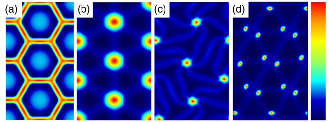
FIG. 22. Spatial plot of the local free energy densities for (a) TH ( \sqrt{3} \times \sqrt{3} ) R30° system at (\varepsilon, W/K) = (3\%, 0.5357 \times 10^{-3}) ; (b) and (c), TT ( \sqrt{3} \times \sqrt{3} ) R30° system at (\varepsilon, W/K) = (3\%, 0.0574 \times 10^{-3}) and (\varepsilon, W/K) = (3\%, 0.1063 \times 10^{-3}) , respectively; and (d) a (1 \times 1) system at (\varepsilon, W/K) = (7\%, 1.997 \times 10^{-3}) . The energy scale from low (blue) to high (red) is shown on the right in arbitrary units.
