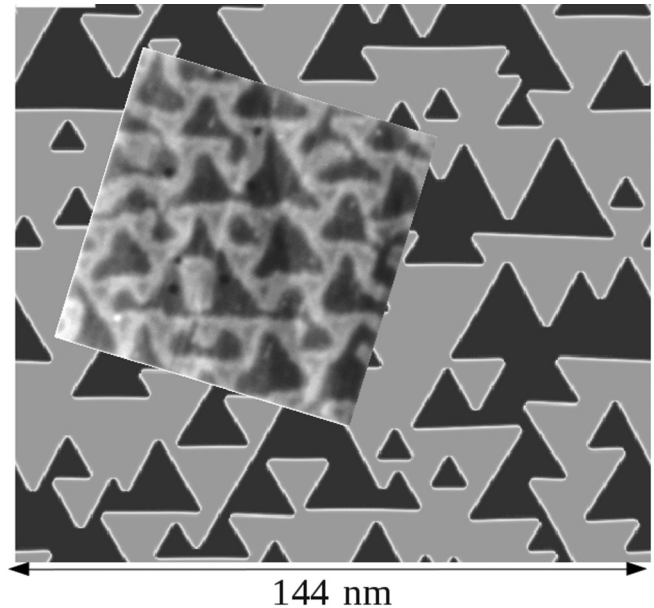
FIG. 23. Comparison between numerically simulated ordering in the large W/K limit for the (1 \times 1) TT system with experimental results of Schmid et al. [27] on the ordering of a partially filled monolayer in the Cu/Ru(0001) system. The experimentally observed pattern is shown as an overlay on a typical configuration (number density plot) from the simulations.
