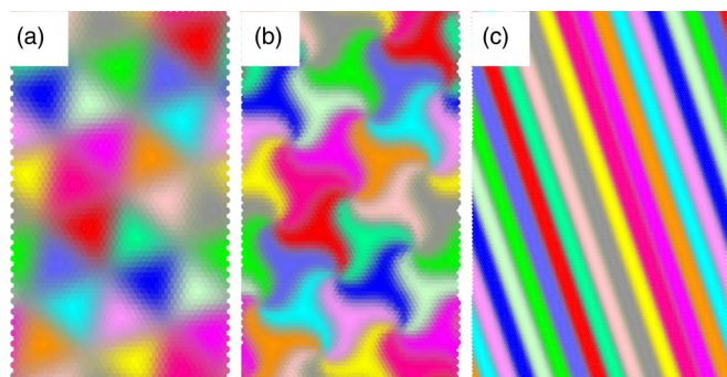
FIG. 19. Sample configurations for the TT (\sqrt{7} \times \sqrt{7})R19.1^\circ case with 2D moiré, twisted 2D moiré, and striped states in (a), (b), and (c), respectively, at \varepsilon = 3\% . Here W/K = 0.0377 \times 10^{-3} , 0.0566 \times 10^{-3} , and 0.377 \times 10^{-3} in (a), (b), and (c), respectively.
