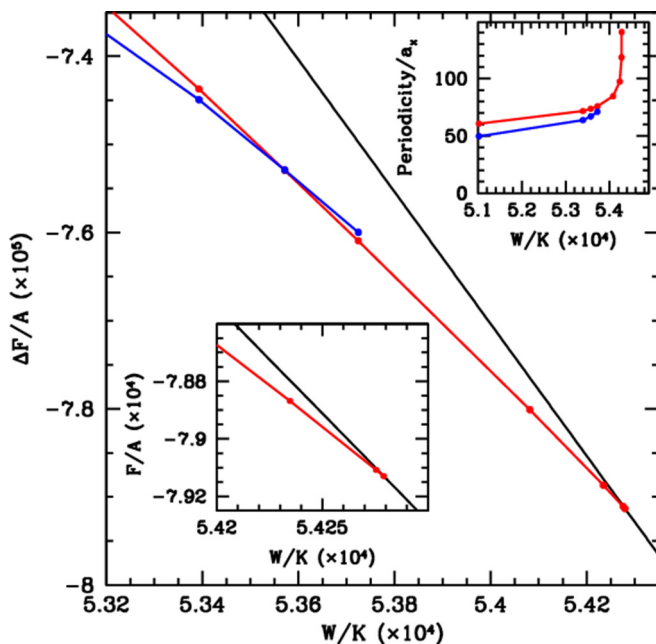
FIG. 11. Free-energy density difference from an incommensurate ( W/K = 0 ) state as a function of W/K for 2D moiré (blue), stripe (red), and commensurate (black) phases at \epsilon = 3\% . In the bottom left inset is a blowup showing that the free energy of the striped phase never becomes higher than that of the commensurate phase indicating a continuous phase transition. In the top inset the periodicity of the 2D moiré (blue) and striped (red) states is shown.
