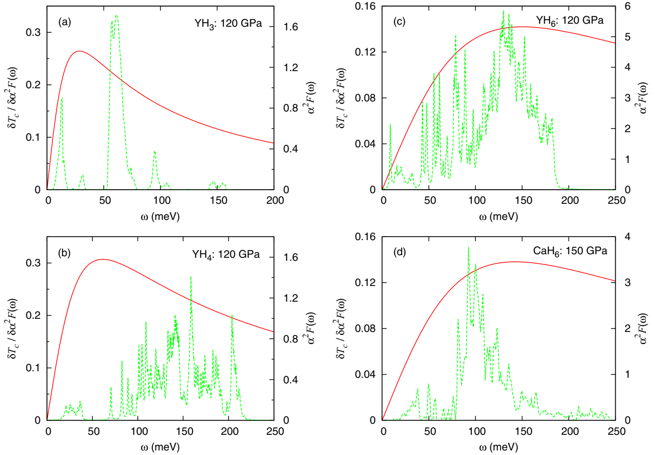
FIG. 2. Functional derivative \delta T_c / \delta \alpha^2 F(\omega) (red solid curve) and the electron-phonon spectral function \alpha^2 F(\omega) (green dashed curve) as a function of frequency \omega for (a) \text{YH}_3 , (b) \text{YH}_4 , and (c) \text{YH}_6 at 120 GPa, and (d) \text{CaH}_6 at 150 GPa.
