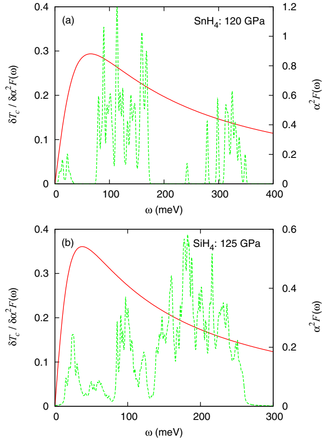
FIG. 1. Functional derivative \delta T_c / \delta \alpha^2 F(\omega) (red solid curve) and the electron-phonon spectral function \alpha^2 F(\omega) (green dashed curve) as a function of frequency \omega for (a) \text{SnH}_4 at 120 GPa and (b) \text{SiH}_4 at 125 GPa.
