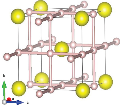
FIG. 3. Crystal structure of \text{H}_3\text{S} .
