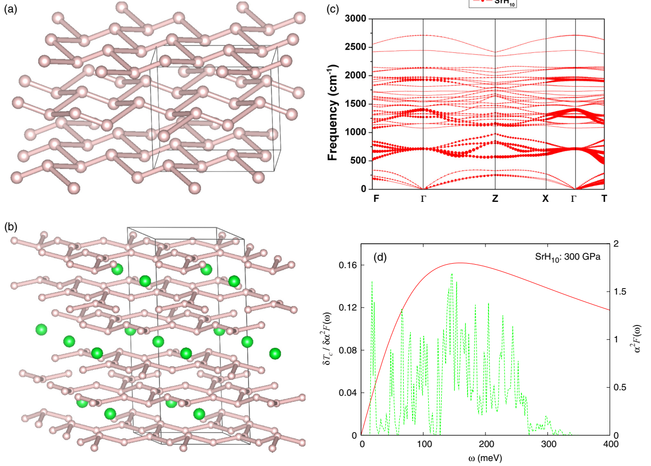
FIG. 4. (a) Cmca structure of molecular hydrogen at 300 GPa, (b) rhombohedral crystal structure of \text{SrH}_{10} , (c) phonon band structure of \text{SrH}_{10} at 300 GPa, and (d) \delta T_c / \delta \alpha^2 F(\omega) (red solid curve) and \alpha^2 F(\omega) (green dashed curve) as a function of frequency \omega for \text{SrH}_{10} at 300 GPa.
