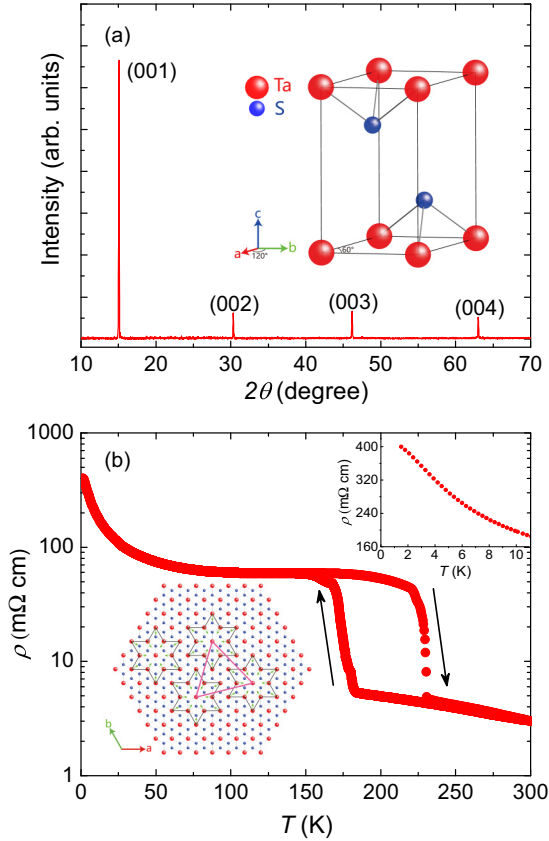
FIG. 1. (a) Room-temperature x-ray diffraction pattern from the large natural surface of the 1T -TaS 2 single crystal. Only (00l) Bragg peaks show up. Inset: Trigonal P\bar{3}m1 crystal structure of 1T -TaS 2 . Ta (S) atoms are displayed by red (blue) balls. (b) Temperature dependence of the resistivity for the 1T -TaS 2 single crystal measured on cooling and warming in zero magnetic field. The hysteresis can be clearly resolved around 200 K, suggesting the occurrence of a first-order phase transition between the NCCDW phase and the CCDW phase. Top right inset: The resistivity in the low- T region. Bottom left inset: A schematic of the monolayer 1T -TaS 2 viewed along the c axis in the CCDW phase. The black line indicates the representative star-of-David clusters, where in-plane Ta atom displacements are marked by green arrows. These star-of-David clusters further form the triangular superlattice (magenta line).
