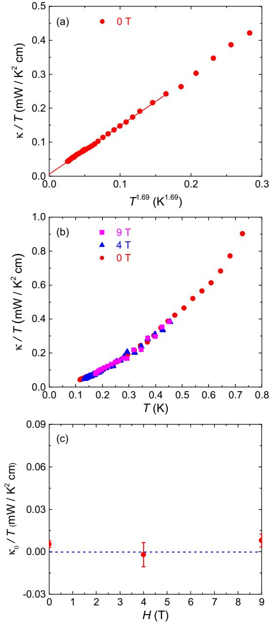
FIG. 2. (a) The in-plane thermal conductivity of the 1T - \text{TaS}_2 single crystal at H = 0 T. The solid line represents the fit of the data to \kappa/T = a + bT^{\alpha-1} . This gives the residual linear term \kappa_0/T = 0.005 \pm 0.002 mW K -2 cm -1 and \alpha = 2.69 . (b) The in-plane thermal conductivity of 1T - \text{TaS}_2 at various magnetic fields ( H = 0, 4, and 9 T) applied along the c axis. (c) Field dependence of the residual linear term \kappa_0/T . The three \kappa_0/T values are negligible in our field range.
