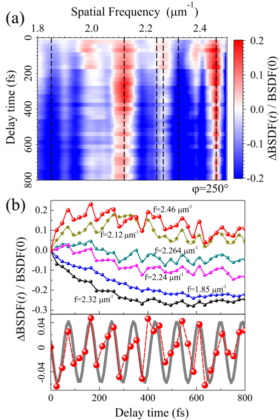
FIG. 10. (a) Transient change \Delta\text{BSDF}(t)/\text{BSDF}(0) of the scattering signal at \varphi = 250^\circ versus spatial frequency of surface relief; F = 6 \text{ mJ/cm}^2 . (b) (Upper panel) The cross sections of the data mapped in (a) along the time axis marked by dashed lines. (Lower panel) The oscillatory part of \Delta\text{BSDF}(t)/\text{BSDF}(0) obtained by high-pass filtering of the signal at f = 2.46 \mu\text{m}^{-1} (circles). Solid line is the fit to equation A_0 \sin(2\pi \nu t + \varphi_0) with \nu = 11.2 THz.
