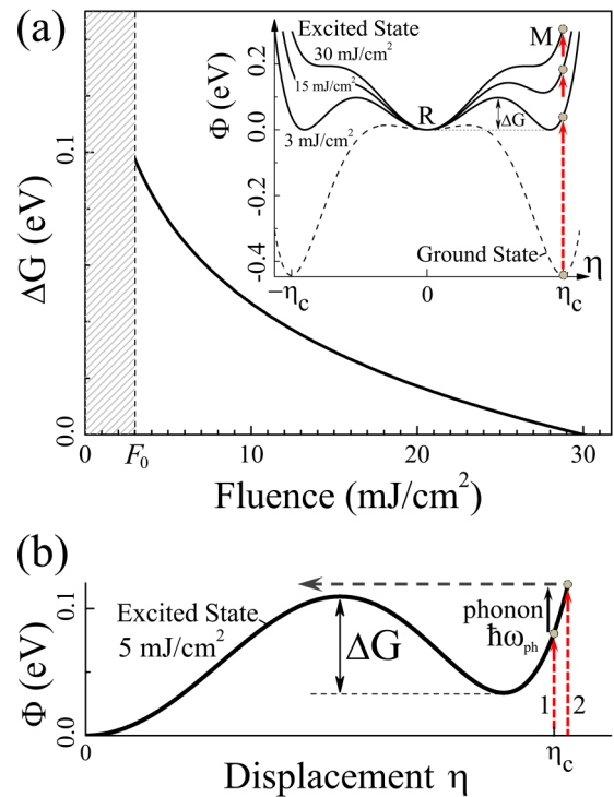
FIG. 13. (a) Potential barrier \Delta G(F) between monoclinic ( M ) and rutile ( R ) phases derived from experimental data using Eq. (5). The inset shows the reconstructed thermodynamic potential \Phi as a function of effective ion displacement \eta for the unperturbed (dashed line curve) and photoexcited (solid line curves) \text{VO}_2 . (b) The photoexcitation of \text{VO}_2 at moderate fluence. The vertical dashed arrow 1 shows the initial under-barrier energy state of the \text{VO}_2 system right after photoexcitation. In this case, the interaction of the system with an optical phonon of frequency \omega_{\text{ph}} results in SPT (shown by horizontal dashed arrow). The vertical dashed arrow 2 indicates the initial over-barrier photoexcited state of \text{VO}_2 . Here the additional energy is gained by the ion subsystem via resonant excitation of Raman modes.
