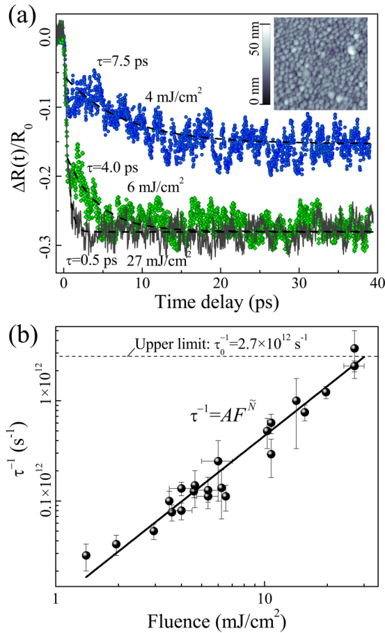
FIG. 12. (a) Transient change of \text{VO}_2/\text{Al}_2\text{O}_3 (C-cut) reflectivity within 40 ps at different levels of optical excitation. Dashed curves are the exponential fit. (Inset) 5 \times 5 \mu\text{m}^2 AFM image of \text{VO}_2/\text{Al}_2\text{O}_3 (C-cut) sample. The average lateral size of grains is 250 nm and rms roughness is 14 nm. (b) The relaxation rate for picosecond component of photoinduced phase transition versus laser pump fluence.
