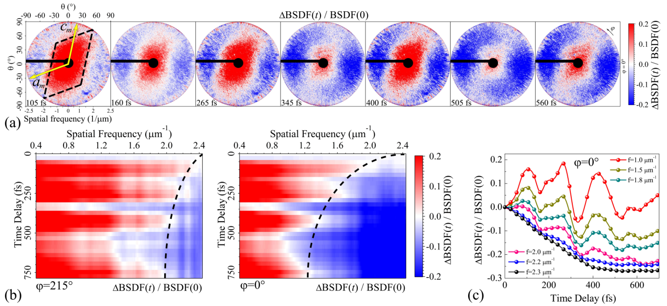
FIG. 8. (a) Transient change \Delta\text{BSDF}(t)/\text{BSDF}(0) of the scattering signal upon light-induced SPT in VO 2 /Al 2 O 3 (A-cut) film; F = 7 \text{ mJ/cm}^2 . Arrows show the orientation of a_m and c_m axes of VO 2 ( M_1 ). Dashed rhomb identifies the oscillatory area of scattering indicatrix. (b) Time-dependent cross sections of the data mapped in (a) at \varphi = 215^\circ and \varphi = 0^\circ versus spatial frequency of surface relief. (c) The cross sections of the data mapped in (b) at \varphi = 0^\circ shows gradual change of oscillatory dynamics versus spatial frequency.
