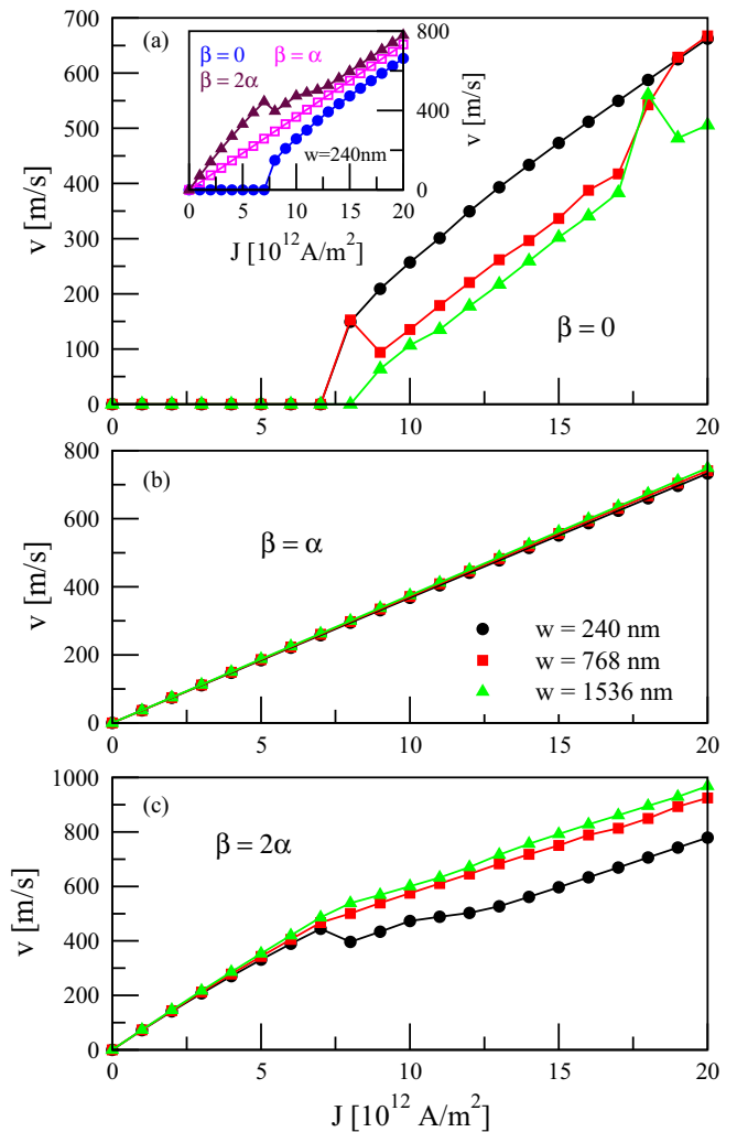
FIG. 6. Main figures: v(J) curves for several values of \beta and different strip geometries, where vortex wall is the equilibrium DW structure. The widths of the strips considered are w = 240 nm, w = 768 nm, and w = 1536 nm. For w = 240 nm the thickness is \Delta_z = 20 nm, whereas for the other two strips \Delta_z = 15 nm. (a) \beta = 0 . Inset: v(J_{\text{ext}}) for a strip with w = 240 nm, \Delta_z = 20 nm, and several values of \beta . (b) \beta = \alpha . (c) \beta = 2\alpha .
