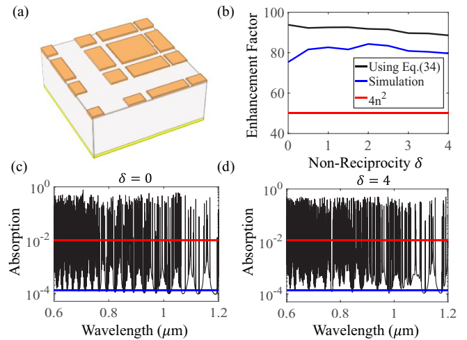
FIG. 3. (a) One unit cell of the solar cell structure considered, with a back-reflector (yellow). The unit cell is a square with side length l = 600 nm, which also corresponds to the periodicity of the structure. The thickness of the bulk absorbing material (grey) is d = 3 \mu\text{m} . The orange regions are nonabsorbing dielectric material. The air slots between the orange regions have widths that are 20%, 5%, and 2% of the period along one direction, and 20%, 5%, and 6% of the period along the other. The thickness of the patterning region is 50 nm. (b) Enhancement factor as a function of the strength of nonreciprocity. The black solid curve was obtained using Eq. (34), which presents the theoretical upper limit of enhancement. The blue curve is the result of our numerically obtained absorption enhancement averaged over the wavelength range of interest and over the two polarizations. The 4n^2 limit is shown in red for reference. (c) and (d) Absorption spectra with spectrally averaged absorption, i.e., \bar{f}(\delta)\alpha_0(\delta)d (red) and single-pass absorption, i.e., \alpha_0(\delta)d (blue) for \delta = 0 and \delta = 4 respectively.
