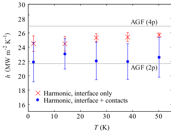
FIG. 7. Conductance in the harmonic system calculated from NEMD using the lead temperatures extrapolated to the interface (red crosses) and the bath temperatures (blue circles) compared with two-probe (2p) and four-probe (4p) AGF calculations.
