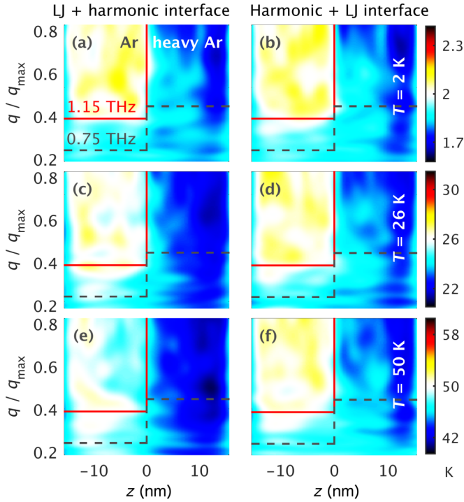
FIG. 4. The same as Fig. 3, but with different forces between atoms at the interfaces. The left panels [(a), (c), and (e)] are calculated from LJ systems with harmonic interfacial forces, and the right panels [(b), (d), and (f)] are from harmonic systems with LJ interfacial forces.
