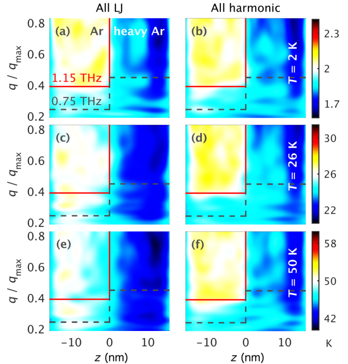
FIG. 3. Distributions of kinetic energy in longitudinal \langle 001 \rangle modes obtained by a wavelet transform during NEMD simulations between Ar ( z < 0 ) and heavy Ar ( z > 0 ). Modes with frequency 0.75 THz are marked with dashed gray lines; modes with frequency 1.15 THz, the maximum frequency in heavy Ar, are marked in solid red. The nominal temperature increases from top to bottom: [(a) and (b)] 2, [(c) and (d)] 26, and [(e) and (f)] 50 K. The left panels [(a), (c), and (e)] are calculated from systems with all LJ forces and the right panels [(b), (d), and (f)] from systems with all harmonic forces.
