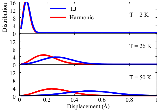
FIG. 6. Average displacements of Ar atoms from their equilibrium positions during NEMD simulations used to calculate conductances in Fig. 2. Distributions were calculated from atoms within the twelve monolayers nearest the interface in six simulations: one simulation with all LJ forces (blue) and one with all harmonic forces (red) at each of three temperatures: 2 (top), 26 (center), and 50 K (bottom).
