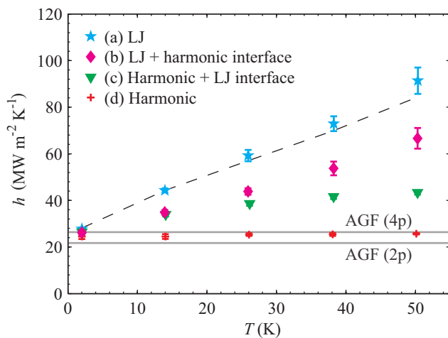
FIG. 2. Thermal boundary conductance as a function of temperature in the same systems as in Fig. 1. Also shown are conductance values calculated using atomistic Green’s functions to model two-probe and four-probe measurements (solid gray). The dashed gray line is the sum of the harmonic conductance of case (d) with the “excess” conductances from cases (b) and (c).
