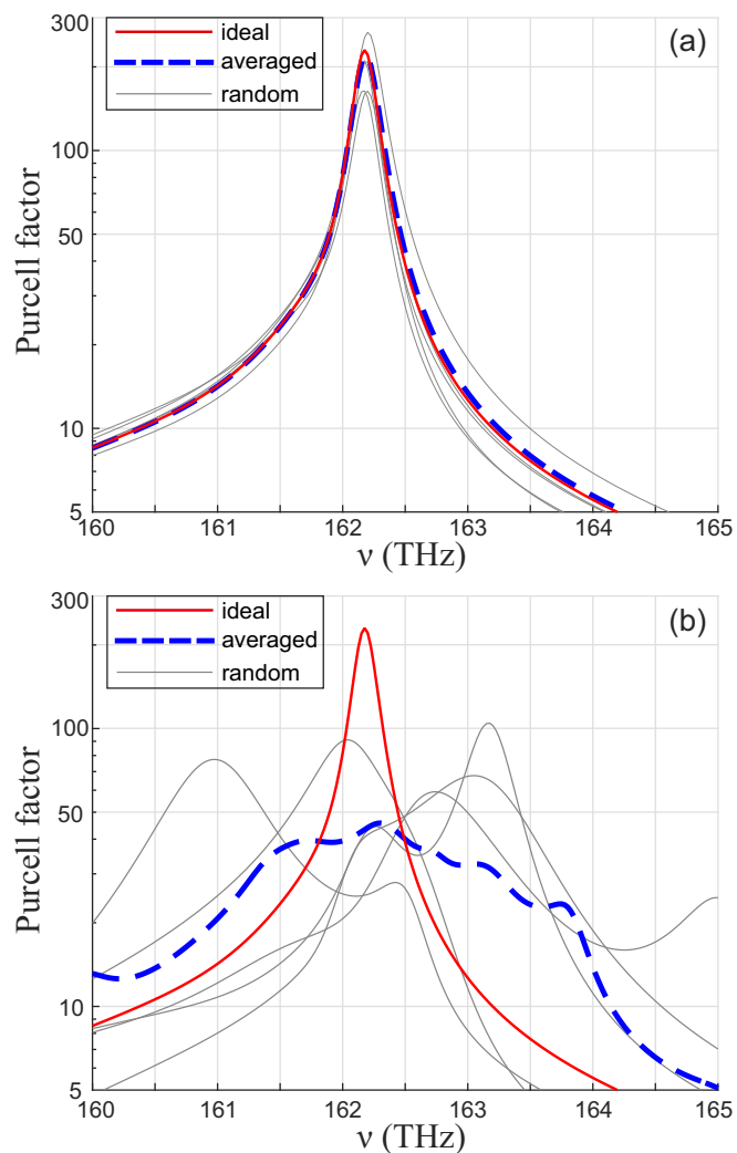
FIG. 11. Purcell factor for the chain of eight core-shell nanoparticles with small random deviations (a) in their positions and (b) in the radii of cores and shells. Parameters of the structure are the same as in Fig. 4(d).
