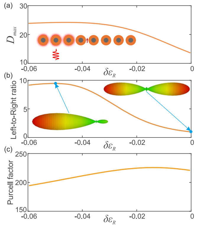
FIG. 5. Tuning of the antenna emission via EHP generation. (a) Directivity, (b) Left-to-right ratio, and (c) Purcell factor for the chain of eight core-shell nanoparticles with a dipole source located in the middle of the chain vs the change in the \text{Re}(\varepsilon_p) of the three leftmost particles. Parameters of the chain are R_c = 82 nm, R_s = 225 nm, and a = 550 nm. Operation frequency is 162.2 THz.
