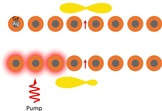
FIG. 1. Schematic of the tunable Yagi-Uda nanoantenna—a periodic chain of metal-dielectric core-shell nanoparticles excited by a dipole emitter. The electric dipole emitter is placed in the center of the chain orthogonally to the chain axis. Generation of electron-hole plasma in the particles at the end of the chain shifts their resonances and dramatically modifies the emission pattern of the nanoantenna.
