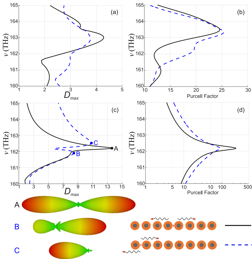
FIG. 4. [(a) and (c)] Directivity and [(b) and (d)] Purcell factor for the chain of 8 core-shell nanoparticles with the dipole source located in the middle of the chain (solid black curves) and between the two leftmost particles (dashed blue curves). (a) and (b) correspond to the R_c = 72 nm radius of Ag core and (c) and (d) to the R_c = 82 nm; the period of the chain is a = 550 nm.
