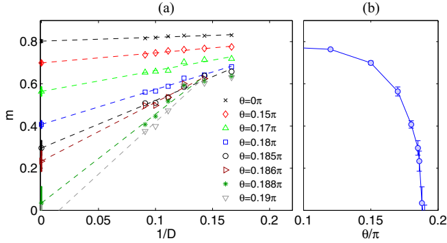
FIG. 2. (a) iPEPS results (full update) for the local magnetic moment m as a function of inverse bond dimension for different values of \theta . (b) Extrapolated values of m as a function of \theta .
