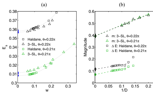
FIG. 4. (a) Energy per site (full update) of the Haldane and three-sublattice (3-SL) state for two different values of \theta , plotted as a function of the truncation error w . (b) Local magnetic moment m (triangles) of the three-sublattice state, and the difference in bond energies \Delta E in the x and y direction in the Haldane state (squares), plotted as a function of 1/D . Note that m and \Delta E are zero in the Haldane and three-sublattice states, respectively.
