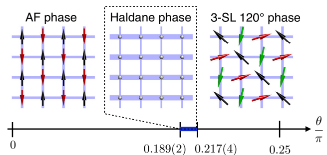
FIG. 1. Haldane phase emerging in between the AF and the three-sublattice 120^\circ ordered phases.
