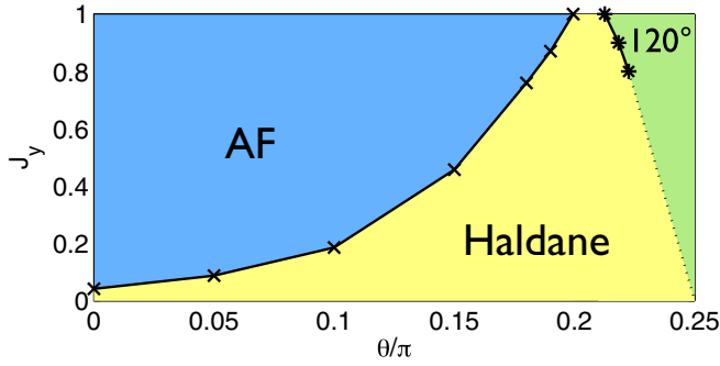
FIG. 3. The phase diagram of the anisotropic bilinear-biquadratic S = 1 model. The phase boundaries were estimated based on D = 10 simple update simulations (see Supplemental Material [71]).
