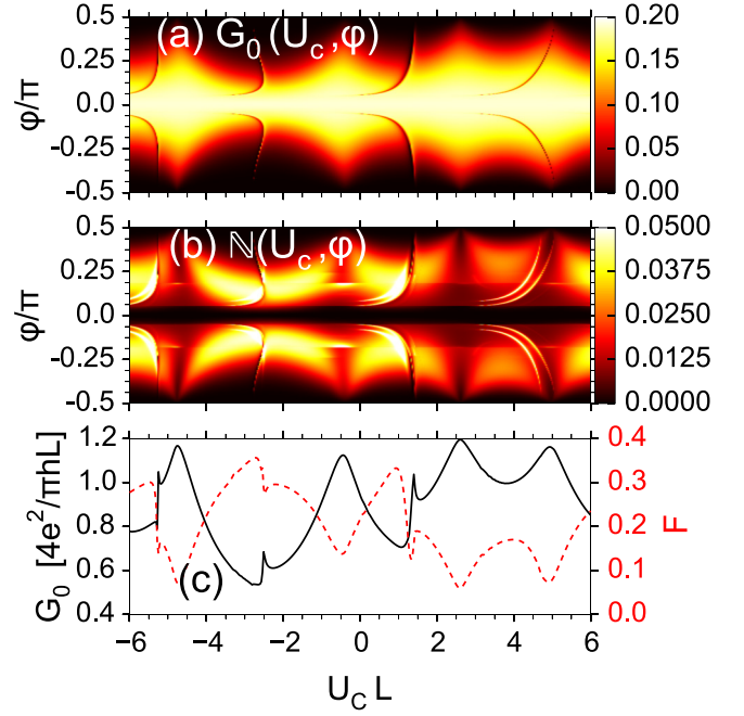
FIG. 4. (a) Angle-resolved dc conductance G_0 , (b) angle-resolved differential shot noise \mathbb{N} , and (c) angle-integrated dc conductance and differential shot noise. The model parameters are Z_0 = 0.4\pi , Z_1 = 0.4 , U = 1.2/L , and \Omega = 1/L .
