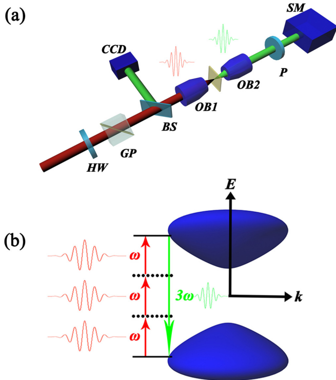
FIG. 1. (a) Experimental setup: the infrared femtosecond laser (red pulse) is tightly focused on the sample by an objective lens (OB1). The induced THG signal (green pulse) is directly measured by a spectrometer (SM). HW is a half-wave plate, GP represents a Glan prism, and P is a polarizer. (b) The diagram illustrates the THG due to the fundamental pulse \omega and the monolayer ReS 2 bandstructure.
