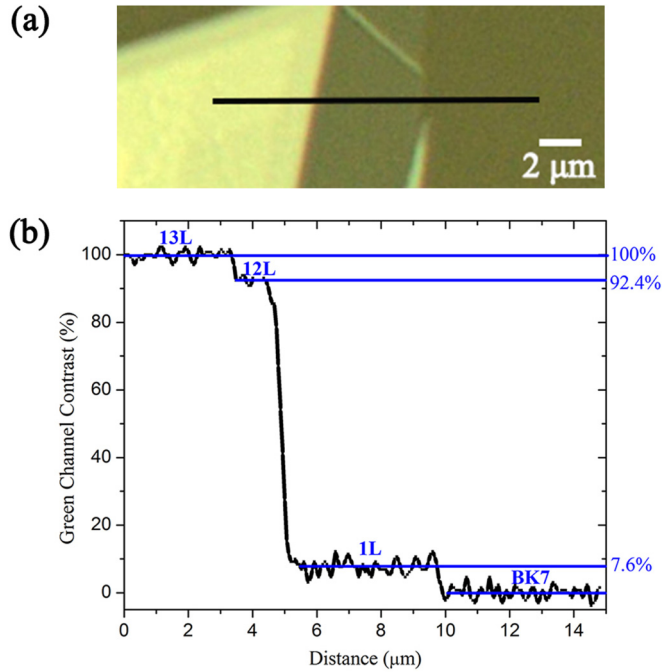
FIG. 3. (a) Zoom-in of the sample region used for optical contrast calculations. (b) Normalized optical contrast of green channel along the black line indicated in (a).
