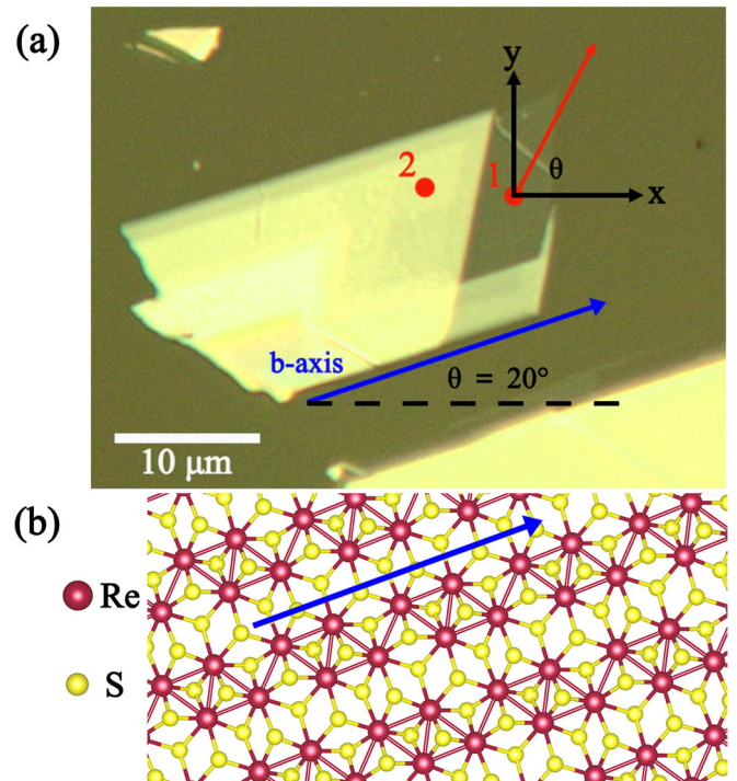
FIG. 2. (a) Microscope image of monolayer ReS 2 and attached multilayer ReS 2 . The red dots 1 and 2 are the laser focusing positions for monolayer and multilayer measurements, respectively. The blue arrow indicates the b -axis direction, which is the direction of the Re atom chains in the lattice. The x and y axes define the laboratory coordinates, and \theta denotes the angle between the polarization direction of the fundamental pulse (red arrow) and the x axis. The angle between b axis of the material and x axis of the laboratory frame is fixed at 20^\circ in the whole study. (b) The distorted 1T lattice structure of ReS 2 , showing the Re atom chain along the b axis (blue arrow).
