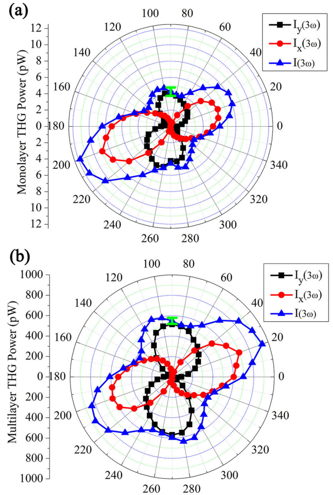
FIG. 6. Angular dependence of THG power in monolayer \text{ReS}_2 (a) and attached multilayer \text{ReS}_2 (b). Horizontal, vertical components of total THG power (blue) are in red and black, respectively. The fundamental pulse power is fixed at 30.2 mW.
