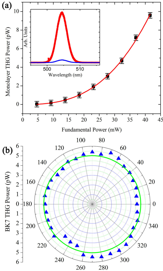
FIG. 5. (a) THG power (black rectangles) of monolayer \text{ReS}_2 as a function of fundamental power. The red line is a cubic fitting. The inset illustrates the third-harmonic spectrum from the monolayer \text{ReS}_2 sample (red) and the BK7 glass substrate (blue) under the same experimental conditions. (b) Angular dependence of THG (blue triangles) in BK7 glass substrate when the fundamental pulse power is fixed at 23 mW. The green line is an isotropic fitting.
