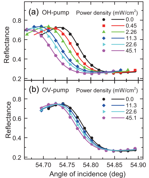
FIG. 3. Results of systematic measurements of the shift of the Fano resonance under (a) OH-pump condition and (b) OV-pump condition. Experimental results are presented by dots and results of Fano fitting are presented by solid curves.
