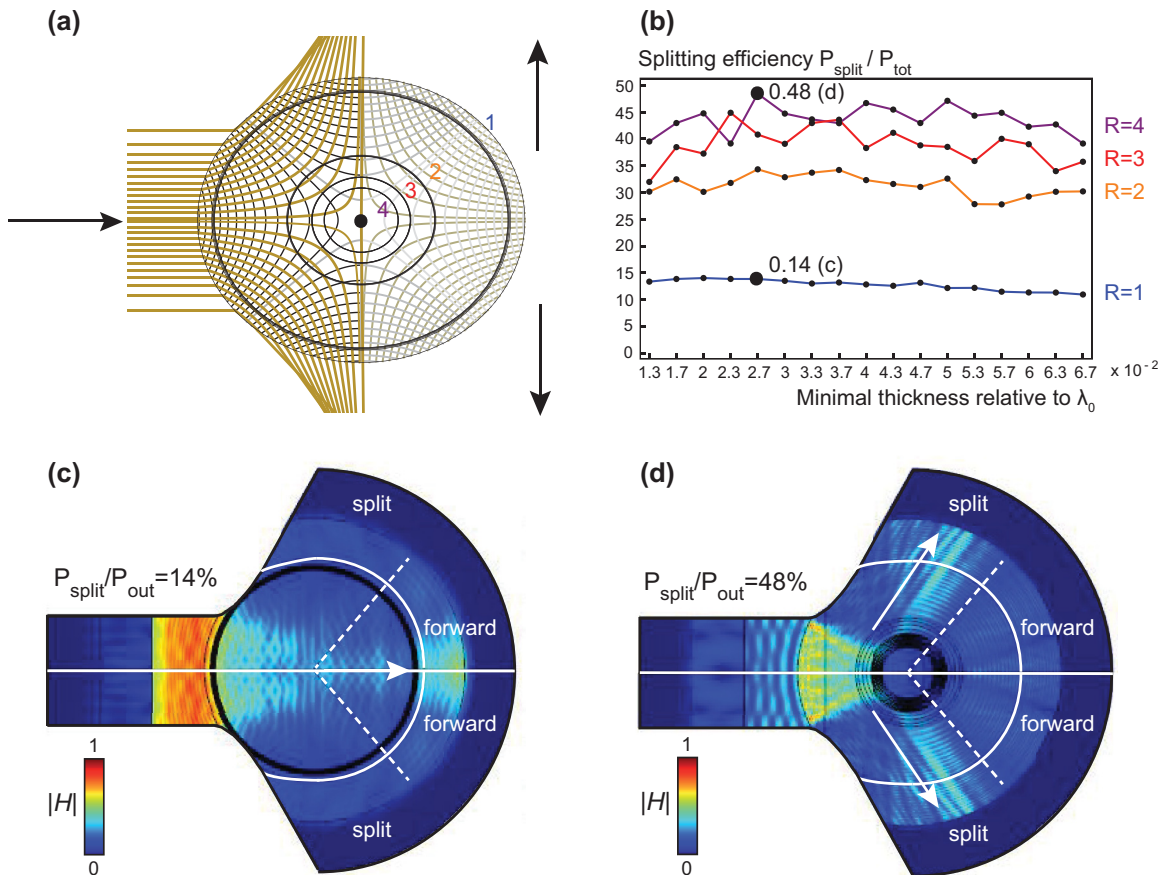
FIG. 3. The effects of a singularity of the first kind on the performance of a metamaterial waveguide, based on a power map w = Rz^2 , for a guided mode corresponding to a free-space wavelength of 1.5 \mu\text{m} and initial waveguide thickness of 2a = 0.4 \mu\text{m} . (a) Light-ray trajectories, obtained from transformation optics, split when approaching the singularity. Truncations impose constant minimal anisotropies within the black circles corresponding to different scaling parameters R and minimal thicknesses a_{\text{min}} . (b) The efficiency, defined in terms of the power P_{\text{split}} that is split and the total power P_{\text{tot}} that comes out of the waveguide, largely depends on the scaling parameter R , while it is almost insensitive to the minimal thickness. (c) When R is equal to one, the norm of the magnetic field coming from the left does not change direction as the embedded transformation in the white circle is almost entirely truncated (disk within the gray-dashed circle). (d) With a large scaling ( R = 4 ), the magnetic norm splits efficiently because the transformation is implemented in regions closer to the singularity. It is only truncated inside the gray-dashed circle with a reduced radius. The power flow, which is proportional to the square of the magnetic norm, is highlighted by the white arrows.
