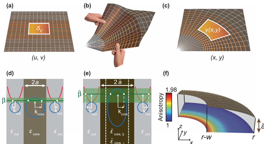
FIG. 1. Materialization of coordinate-transformed guided waves with a uniaxial waveguide core ( \tilde{\epsilon}_{\parallel}, \tilde{\epsilon}_{\perp} ) and a thickness variation \tilde{a} based on Ref. [27]. (a)–(c) A two-dimensional conformal transformation transforms (a) straight light flows (orange lines) along a trivial dielectric slab waveguide into (c) curved ones by inducing a geometry component \gamma(x, y) on the waveguide plane. (d) The initial guided mode along a slab waveguide with thickness 2a and permittivities \epsilon_{\text{core}} ( \epsilon_{\text{out}} ) in the core (outer regions) is fully characterized by an in-plane propagation constant \beta (green line) parallel to the waveguide plane at a particular angular frequency \omega . Indeed, it determines the characteristic variations of the transverse profile, i.e., the sinusoidal variations inside the core [ \cos(k_{\text{core}}z) ] correspond to the intersection of the green line with the blue ellipse, while the exponentially decaying fields outside of the core [ \exp(-|k_{\text{out}}z|) ] correspond to the intersection of the green line with the red hyperbola. (e) The coordinate transformation stretches the in-plane propagation constant \tilde{\beta} along the waveguide plane, which is implemented by a uniaxial material inside the core ( \tilde{\epsilon}_{\parallel}, \tilde{\epsilon}_{\perp} ). To ensure that boundary conditions are compatible with \tilde{\beta} , the thickness \tilde{a} has to change according to Eq. (1). (f) A visualization of the beam bender design in Ref. [27] shows that the anisotropy of the core is modest and highest at the inner radius of the bend (surface coloring on the waveguide symmetry plane). The thickness variation \tilde{a} is visualized by the gray floating surface, representing the upper interface of the waveguide. Subsets of this figure have been reproduced from Ref. [27].
