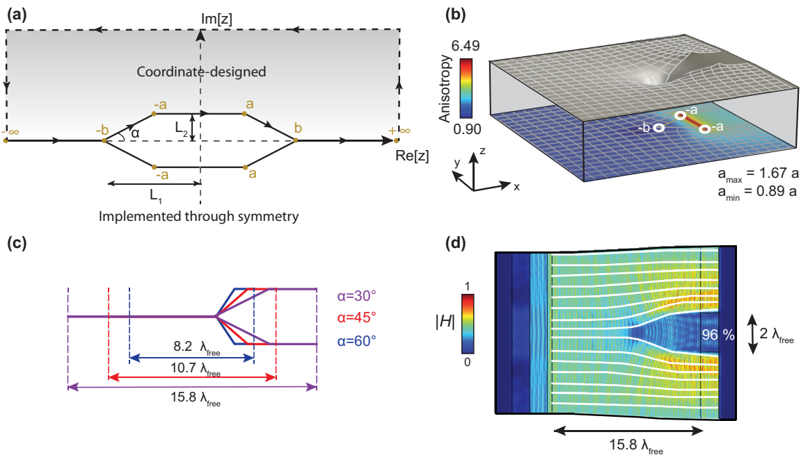
FIG. 4. A beam-splitter design based on a Schwarz-Christoffel transformation: (a) Sketch of the polygonal boundary corresponding to a beam splitter and/or interferometer. The coordinate transformation in the lower part of the beam splitter is obtained through symmetry. (b) The extremal values of the in-plane components of the geometry (surface coloring on the waveguide's symmetry plane) and the symmetric thickness variation (floating surface) clearly allow identification of the locations of the vertices corresponding to -b and -a . (c) Identical separations may be obtained with different splitting angles \alpha = 30^\circ (purple), \alpha = 45^\circ (red), and \alpha = 60^\circ (blue) and splitting lengths. (d) The magnetic norm (surface coloring) and the power flow (white lines) behave as expected, splitting after the initial vertex with an efficiency P_{\text{split}}/P_{\text{tot}} of 96% for a splitting angle of 30 degrees.
