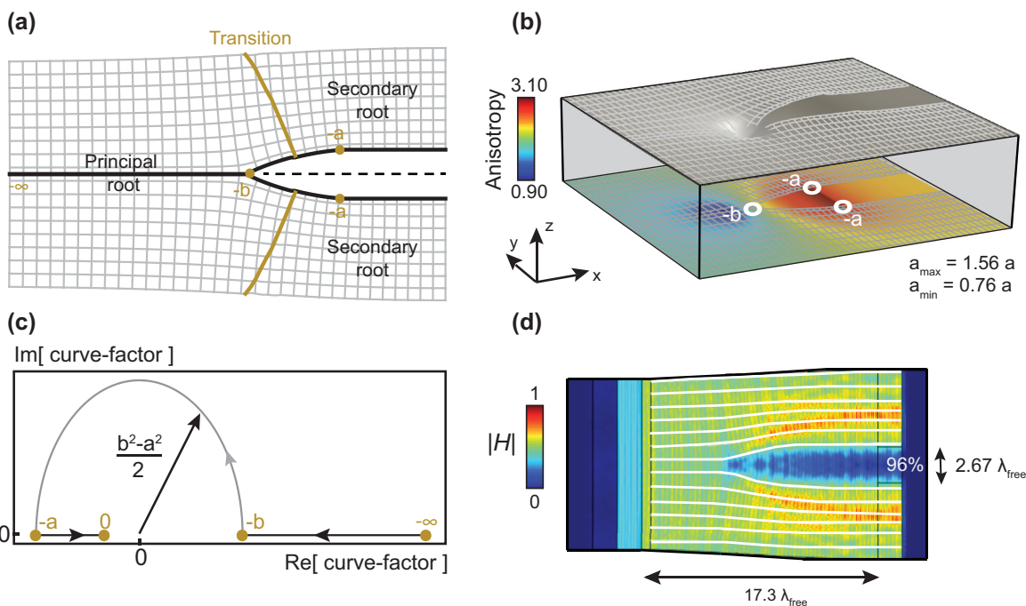
FIG. 5. A beam-splitter design with curve factors requires much more moderate optical parameters, i.e., the anisotropy is reduced by a factor of two. (a) The transformation generates a continuous geometry by making use of two Riemann surfaces, separated by the yellow line, corresponding to different signs of the square root in the curve factor. (b) The geometry (surface coloring on symmetry plane) and thickness variation of the upper interface (gray floating surface) occur in a more gradual and less extreme way than those of conventional Schwarz-Christoffel designs [Fig. 4], at the expense of a longer splitting length. (c) The curve factor induces a phase change from 0 to \pi on the edge [-b, -a] at a constant magnitude. (d) Full-wave simulations of the magnetic norm (surface coloring) and the power flow (white lines) demonstrate that the beam splitter splits with an efficiency of 96.4%, comparable to the efficiency of the conventional Schwarz-Christoffel transformation.
