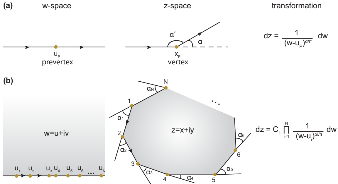
FIG. 2. A Schwarz-Christoffel transformation generates (a) vertices or (b) polygonal boundaries with a series of power maps between the complex w and z plane. This is achieved by making use of local power maps with exponents 1 - \alpha/\pi (right-hand side).
