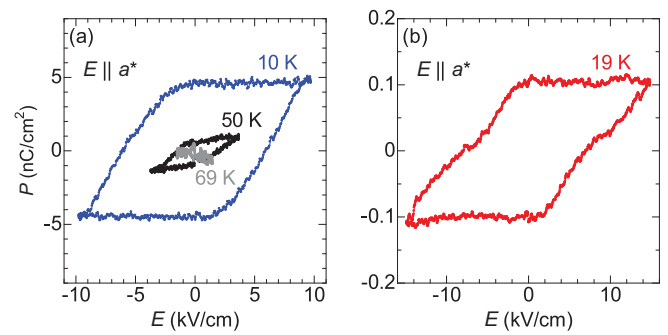
FIG. 3. Electric-field dependence of polarization along the a^* axis measured using the PUND method (a) at 10, 50, and 69 K and (b) at 19 K for another sample.
