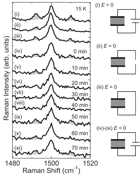
FIG. 2. Raman spectra of ( cc ) at 15 K and schematics for four experimental configurations. (i): An electric field of 5 kV/cm was applied. (ii) Voltage source was decoupled. (iii) Shunt after (ii). (iv)–(xi) -5 kV/cm was applied.
