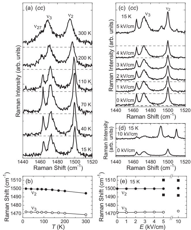
FIG. 1. (a) Temperature dependence of the Raman spectra in ( cc ) for \beta' -(BEDT-TTF) _2 ICl _2 . Here, ( cc ) denotes that the polarizations of the incident light and the detected light were both set parallel to the c axis. (b) Raman shifts of the \nu_2 and \nu_3 modes plotted against temperature. (c) Electric-field dependence of the Raman spectra in ( cc ) at 15 K. The electric field (0–5 kV/cm) was applied parallel to the b' axis. (d) Raman spectrum at 15 K under 10 kV/cm compared with that without the electric field. (e) Raman shift of the \nu_2 and \nu_3 modes plotted against applied electric field at 15 K. In (b,e), filled and open symbols show the \nu_2 and \nu_3 modes, respectively. Circles are the original peaks, and squares are the field-induced peaks.
