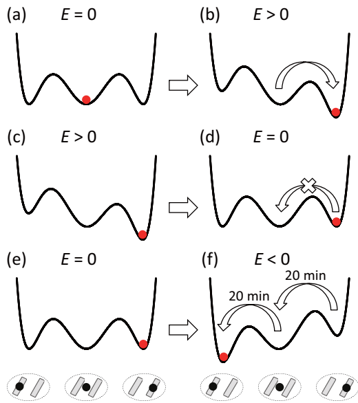
FIG. 4. Schematics of the three-valley model. The center valley indicates the Mott insulating state, in which the charge is equally distributed to the two constituent BEDT-TTF molecules. The right and left valleys indicate the charge-disproportionate states. The right one corresponds to the state in which the charge is located in the right BEDT-TTF molecule. In the left valley, the charge is located in the left molecule.
