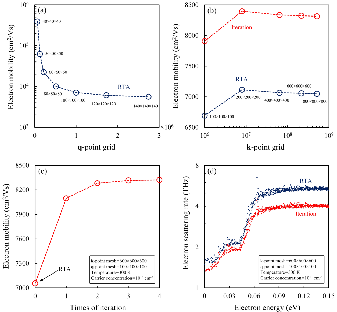
FIG. 1. (a) Electron mobility computed by a fixed 600 \times 600 \times 600 \mathbf{k} -point mesh with respect to varying density of \mathbf{q} -point grids. (b) Electron mobility computed by a fixed 100 \times 100 \times 100 \mathbf{q} -point mesh with respect to varying density of \mathbf{k} -point grids. The blue and red circles are the mobilities calculated from the RTA and iterative scheme, respectively. (c) Evolution of electron mobility with respect to times of iteration. (d) Electron scattering rates near the \Gamma point. The blue and red dots are the scattering rates computed by using the RTA and iterative scheme, respectively, from the 600 \times 600 \times 600 \mathbf{k} -point and 100 \times 100 \times 100 \mathbf{q} -point meshes. The studied temperature and carrier concentration in these simulations as shown in the four panels are 300 K and 10^{13} \text{ cm}^{-3} , respectively.
