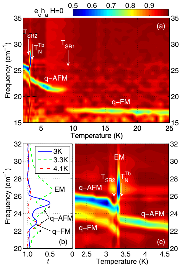
FIG. 1. (a) Normalized transmittance map of \text{TbFeO}_3 measured in the e_c h_a configuration at temperatures from 2.2 to 25 K. (b) Spectra of transmittance t for temperatures above (4.1 K), at (3.3 K), and below (3 K) the temperature of Tb magnetic ordering T_N^{\text{Tb}} \approx 3.3 K. (c) An expanded view of the rectangular region in (a) showing the behavior of q-AFM, q-FM, and EM excitations in the vicinity of Tb magnetic ordering.
