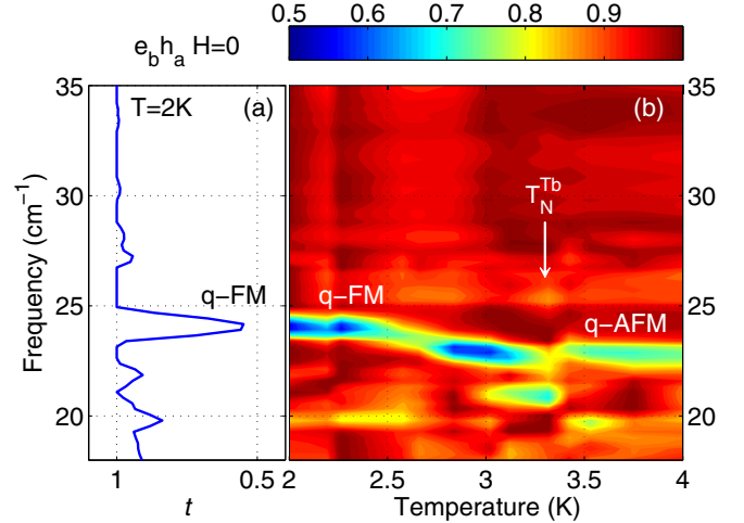
FIG. 2. (a) Normalized transmittance spectrum t of \text{TbFeO}_3 measured in the e_b h_a configuration at T = 2 \text{ K} < T_N^{\text{Tb}} and H = 0 . (b) Normalized transmittance map manifesting q-FM excitation below T_N^{\text{Tb}} and q-AFM one above T_N^{\text{Tb}} .
