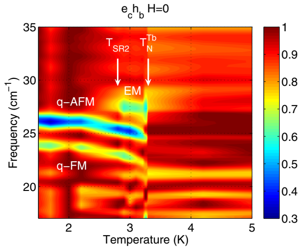
FIG. 3. Temperature dependence of the normalized transmittance of TbFeO 3 measured in the e_c h_b configuration at H = 0 manifesting q-AFM, q-FM, and EM excitations below T_N^{\text{Tb}} . Electromagnon EM is visible in a narrow temperature region between T_{\text{SR}2} and T_N^{\text{Tb}} .
