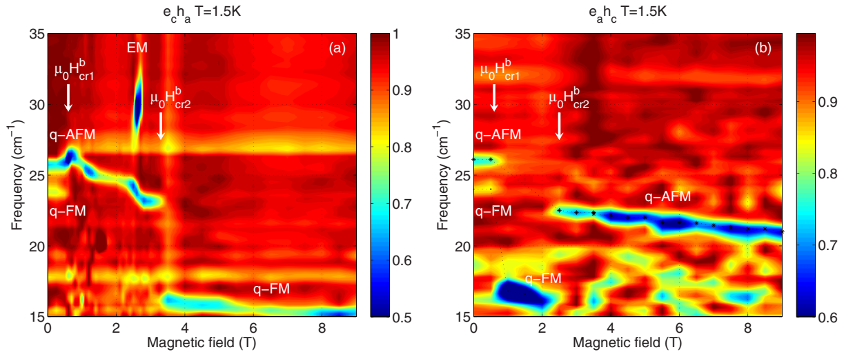
FIG. 5. Magnetic-field dependence ( H\parallel b ) of normalized transmittance measured in the e_c h_a (a) and e_a h_c (b) configurations at T = 1.5 K
