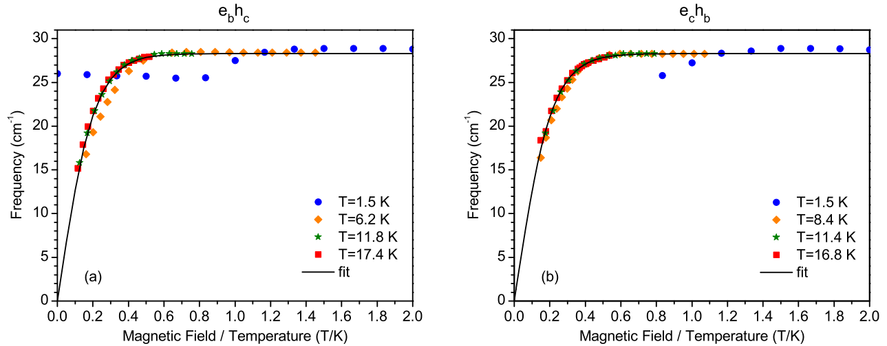
FIG. 8. Experimental data for the q-FM mode's frequency measured in the e_b h_c (a) and e_c h_b (b) configurations in the magnetic field H \parallel a presented as a function of \mu_0 H_a / T .
