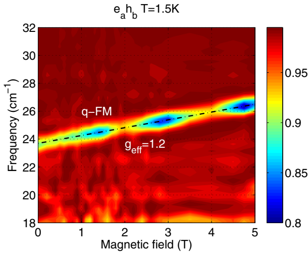
FIG. 7. Magnetic-field dependence ( H\parallel c ) of normalized transmittance measured in the e_a h_b configuration at T = 1.5 K.
