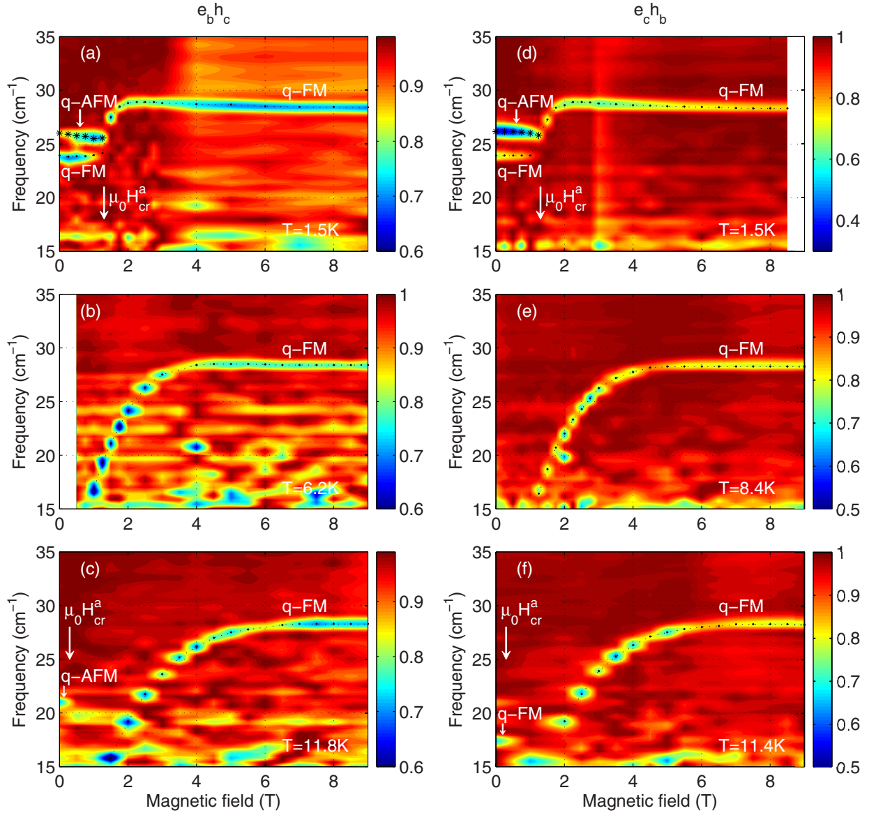
FIG. 4. Magnetic-field dependence ( H\parallel a ) of normalized transmittance measured in the e_b h_c configuration at (a) 1.5 K, (b) 6.2 K, and (c) 11.8 K and in the e_c h_b configuration at (d) 1.5 K, (e) 8.4 K, and (f) 11.4 K.
