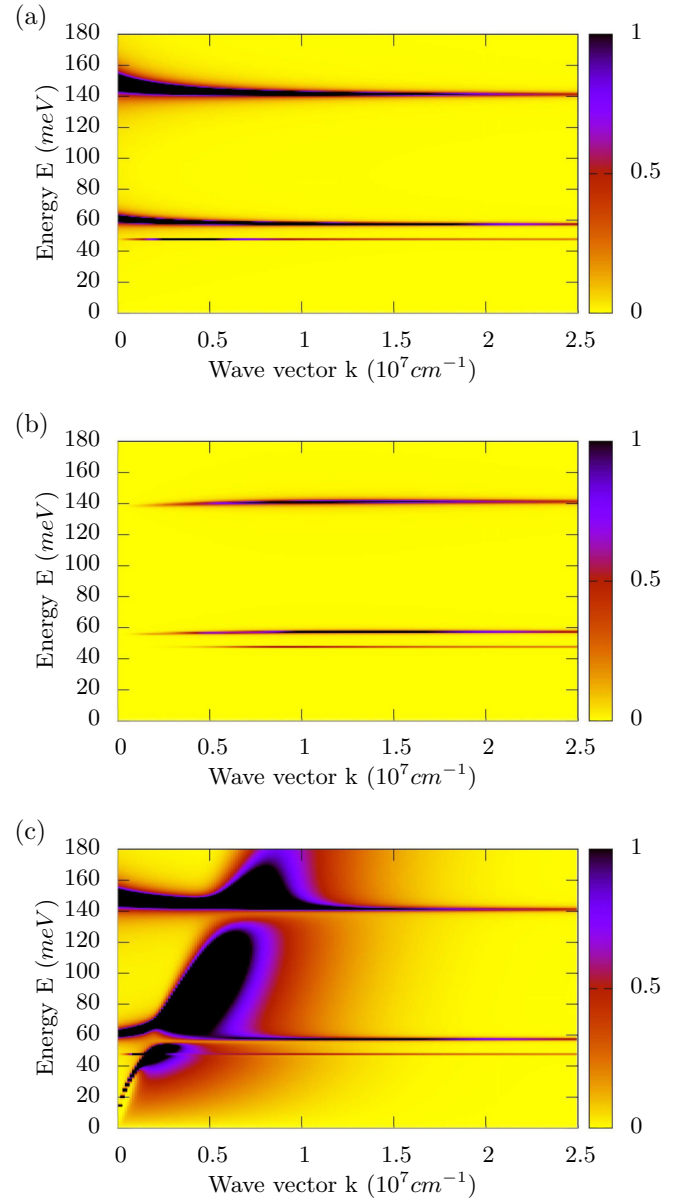
FIG. 11. \Im m\left(\frac{-\epsilon^\infty}{\epsilon^c + \epsilon_{\text{interface}} - \epsilon^\infty}\right) \propto W_{k,\omega}^0/v_k Eq. (57) in the \text{SiO}_2\text{-MoS}_2\text{-vacuum} structure at T = 300\text{ K} and n = 2 \times 10^{12}\text{ cm}^{-2} , as a function of wave vector k and energy E = \hbar\omega , with different treatments of screening: (a) no screening \epsilon^c = 0 , (b) static screening \epsilon^c = \epsilon^c_{k,\omega=0} and (c) dynamic screening \epsilon^c = \epsilon^c_{k,\omega=0} .
