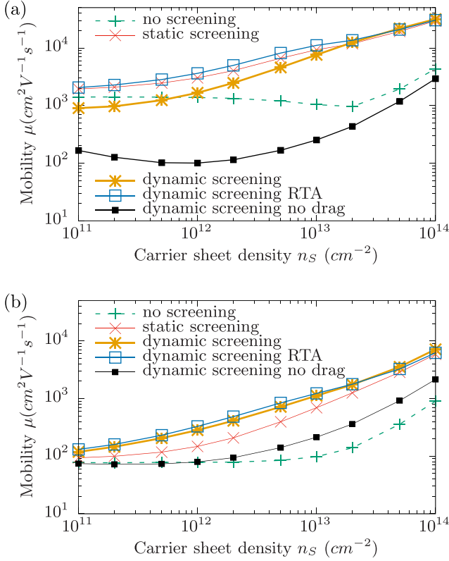
FIG. 10. Room-temperature mobility limited by interface phonon- plasmon scattering in the (a) \text{SiO}_2\text{-MoS}_2\text{-vacuum} and (b) \text{HfO}_2\text{-MoS}_2\text{-SiO}_2 structures as a function of carrier sheet density n_s . Sec. VB 2 explains how the mobilities tagged “no screening,” “dynamic screening,” “dynamic screening RTA,” “dynamic screening no drag,” and “static screening” are calculated.
