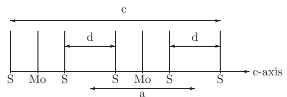
FIG. 7. Projection of the \text{MoS}_2(2\text{H}) primitive unit cell onto the c axis, to scale. Lines perpendicular to the c -axis mark the planes in which the marked atoms sit. The length of the unit cell is c = 12.29 \text{ \AA} , the interatomic distance is d = 2.96 \text{ \AA} [48]. The size of a unit cell of a monolayer a = c/2 = 6.145 \text{ \AA} .
