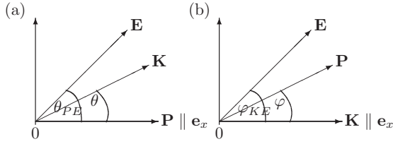
FIG. 19. Coordinate system for (a) \mathbf{K} integral in \tau_P , Eq. (D4), and (b) \mathbf{P} integral in T_{\mathbf{K},\Omega} , Eq. (D10).
