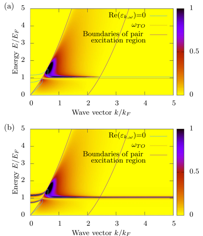
FIG. 1. \Im m\left(-\frac{1}{\varepsilon_{k,\omega}^{\text{tot}}}\right) in GaAs at T = 0 and n = 5 \times 10^{17} \text{ cm}^{-3} with an anharmonic optical phonon damping rate (a) \gamma = 0 , and (b) \gamma = 0.007\omega_{\text{TO}} , as a function of wave vector k and energy E = \hbar\omega .
