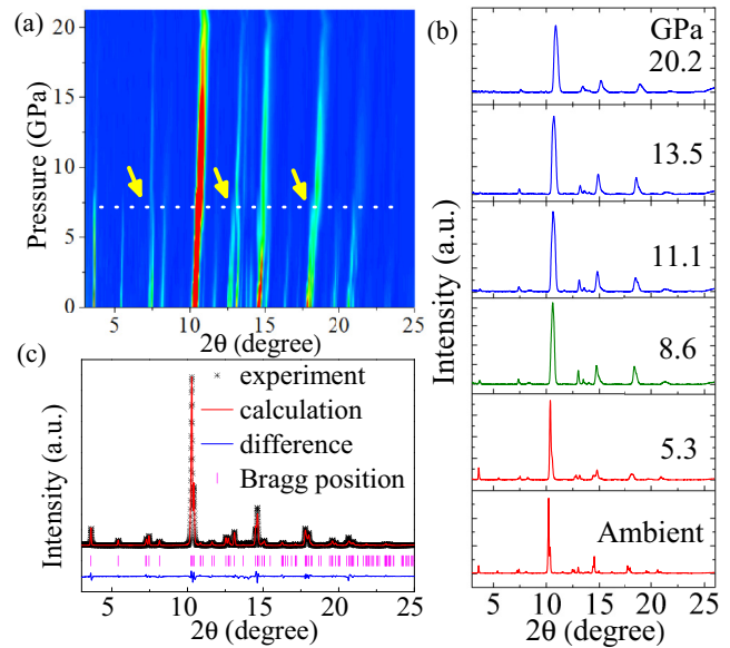
FIG. 4. Pressure-dependent x-ray diffraction patterns. (a) 2D XRD pattern; yellow arrows are plotted to show the phase transition. (b) Selected XRD patterns at various pressures (ambient conditions, 5.3 GPa, 8.6 GPa, 11.1 GPa, 13.5 GPa, and 20.2 GPa). (c) XRD refinement (ambient conditions).
