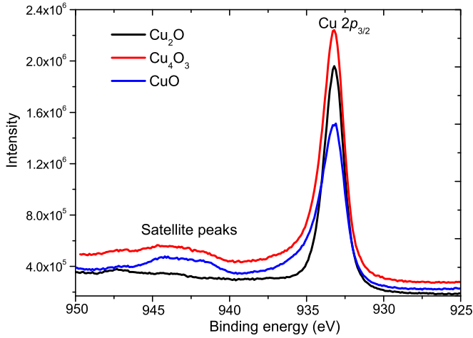
FIG. 4. Cu 2p_{3/2} core-level XPS spectra of \text{Cu}_2\text{O} , \text{Cu}_4\text{O}_3 , and CuO thin films.
