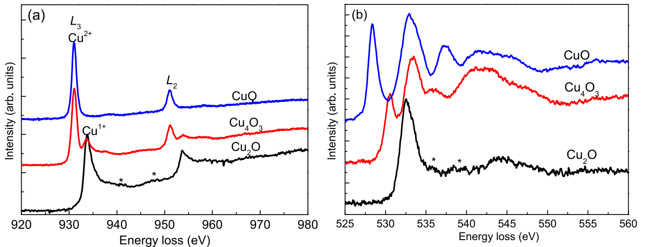
FIG. 5. (a) Cu L_{2,3} edges and (b) O K edge ELNES spectra of \text{Cu}_2\text{O} , \text{Cu}_4\text{O}_3 , and CuO, normalized to the peak height.
