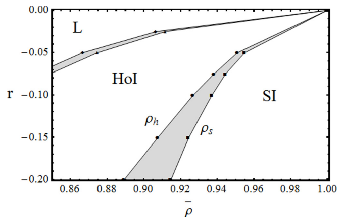
FIG. 1. Phase diagram showing the striped incommensurate phase (SI), honeycomb incommensurate phase (HoI), and the co-existence region (dark area) in the range \rho_h < \bar{\rho} < \rho_s . L corresponds to a uniform phase without domain-wall patterns.
