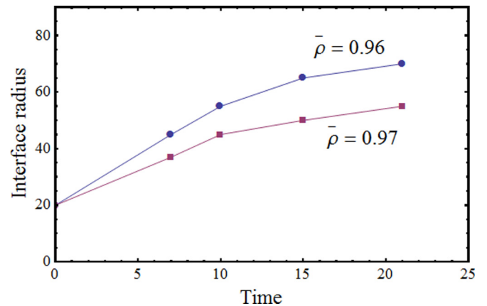
FIG. 4. Radius of the expanding SI-HoI interface as a function of time (in units of 4.8 \times 10^5 dt ) for initial stripe phases with different average densities \bar{\rho} , for a hole of radius R = 20dx .
