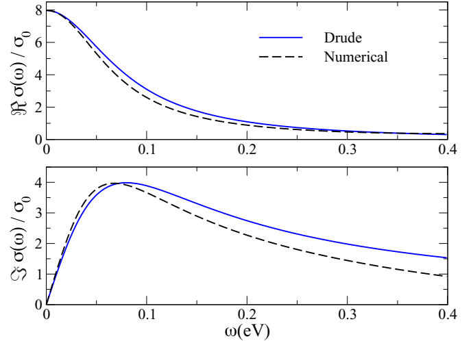
FIG. 3. Fit of numerical optical conductivity data with the Drude model for \mu = 0.5 eV, where \hbar/\tau = 0.07 eV is the adjustable parameter. The spectral weight is given by \sigma_{D,0}(T, \mu) = \frac{2e^2 \tau k_B T}{\pi \hbar} \log [2 \cosh(\frac{\mu}{2k_B T})] .
