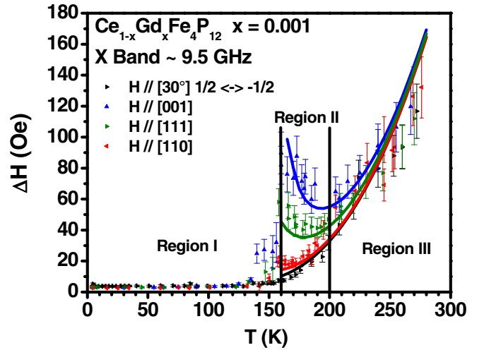
FIG. 5. ESR linewidth of \text{Ce}_{1-x}\text{Gd}_x\text{Fe}_4\text{P}_{12} ( x \approx 0.001 ), triangles represents the experimental results [31]. Region I shows the ESR linewidth of transition -\frac{1}{2} \leftrightarrow \frac{1}{2} for main crystal orientations. Full lines in regions II and III show theoretical simulations of the overall full linewidths of the collapsed spectra, including all ESR transitions.
