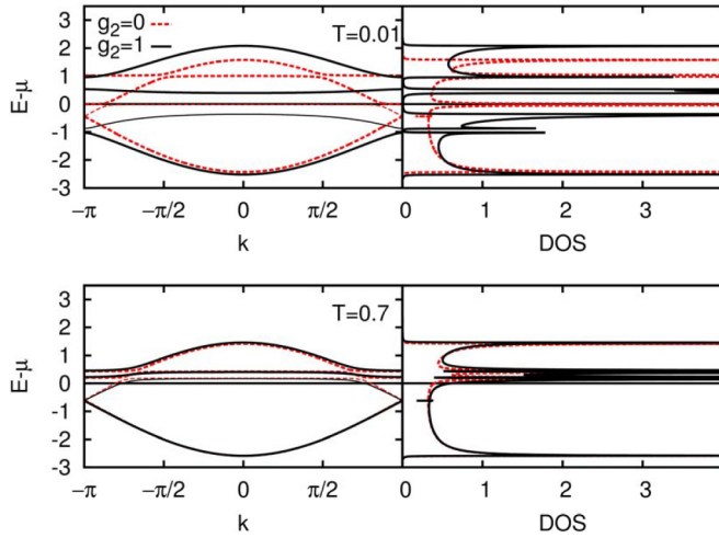
FIG. 3. Dispersion relation (left panels) and corresponding density of states ( \text{DOS} = \frac{1}{\pi} \text{Im}[G(\omega + 0.002I)] , right panel). Full black (dashed red) lines correspond to the coupled (uncoupled) lattice and electron case. Top panels correspond to T = 0.01 . Lower panels correspond to T = 0.7 .
