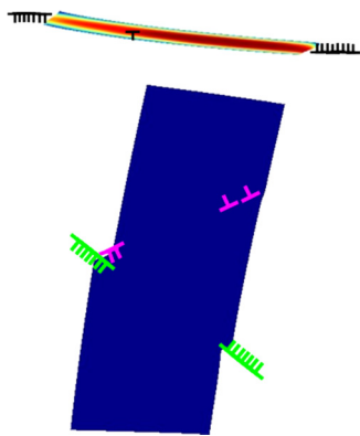
FIG. 24. The phase and dislocations solution at t = 0.75 under p = 5 and \gamma = 0.3 with five times larger L_\xi = 5 \times 10^4 (Pa s) -1 ( L_\eta/L_\xi = 0.052 ). High-pressure phase does not nucleate.
