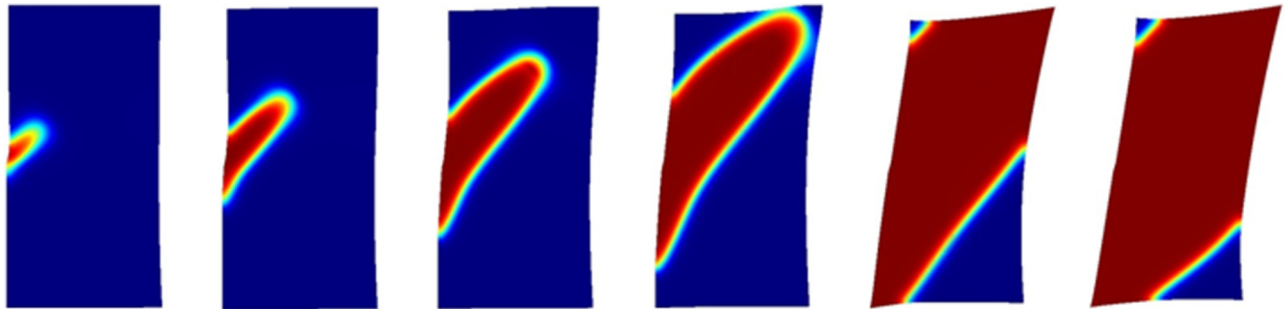
FIG. 2. Evolution of high-pressure phase under the hydrostatic pressure of 15.9 in the presence of a single dislocation.
