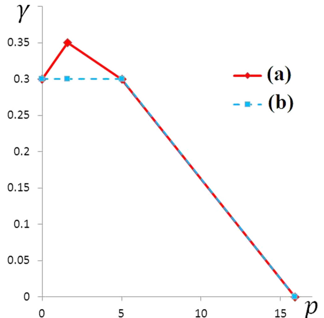
FIG. 23. The minimum applied shear strain vs the applied pressure to nucleate HPP in the right grain: (a) HPP nucleation only at the tip of dislocation pile-up located in the left grain and (b) HPP nucleation at any place in the right grain.
