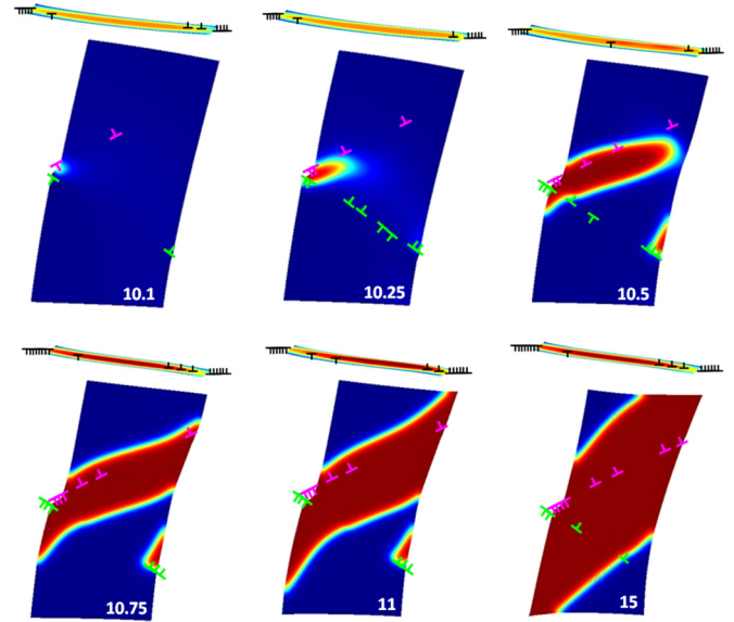
FIG. 11. Evolution of the high-pressure phase and dislocations under p = 5 and \gamma = 0.3 with plasticity in the right grain.
