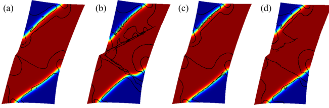
FIG. 16. Stationary phase state and contour lines of the equilibrium transformation work ( \langle \boldsymbol{\sigma} : \boldsymbol{\varepsilon}_t = \Delta^\theta G(\theta) = 0.608 ) for case 1 without (a) and with plasticity (b), and for case 2 without (c) and with plasticity (d).
