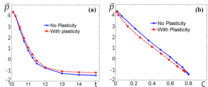
FIG. 9. Pressure averaged over right grain vs time and the concentration of high-pressure phase under p = 1.59 and \gamma = 0.35 in the right grain with and without plasticity. With plasticity, the pressure is higher for the same time but lower for the same concentration of high-pressure phase.
