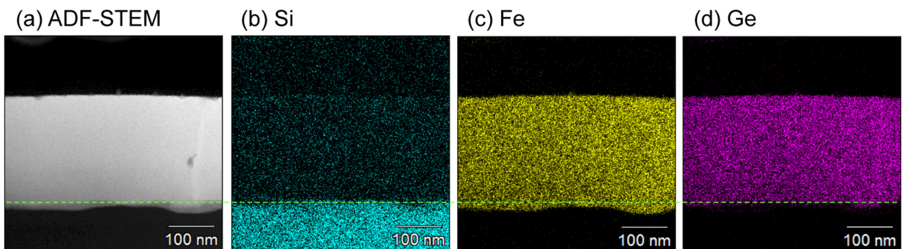
FIG. 5. (a) ADF-STEM image and (b)–(d) EDX mappings for Si, Fe, and Ge elements.
