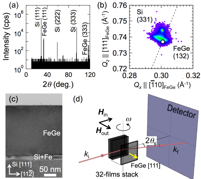
FIG. 1. (a) \theta - 2\theta x-ray diffraction pattern of the FeGe thin film. (b) Reciprocal-space map around the Si (331) peak. The peak position estimated from the lattice parameter of bulk FeGe is indicated by an open circle. (c) Cross-sectional transmission electron microscopy image. (d) Experimental setup for the SANS experiment. The stack of 32 thin films of 15 mm \times 15 mm size are aligned with their surfaces along the incident neutron beam when the rocking angle is zero. Magnetic fields were applied both parallel ( H_{in} ) and perpendicular ( H_{out} ) to the film surfaces.
