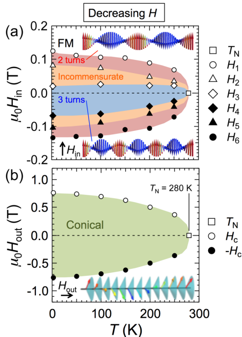
FIG. 4. Magnetic phase diagrams under decreasing (a) H_{in} and (b) H_{out} from large magnetic fields (e.g., H_{in} = 0.25 T and H_{out} = 1.0 T). Schematic illustrations of helicoidal and conical states are inset in panels (a) and (b), respectively.
