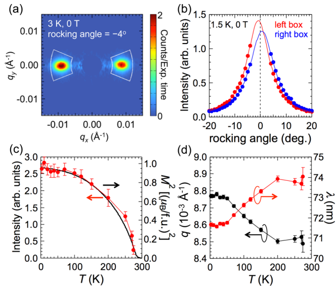
FIG. 2. (a) Typical SANS pattern at zero magnetic field. Due to the strong reflected neutron intensity from the periodic array of Si substrates, the magnetic Bragg scattering is discerned above a small offset rocking angle ( \approx \pm 4^\circ ) [34]. (b) Rocking scan of magnetic Bragg peaks. Intensities in the left and right boxes in panel (a) are indicated by red and blue markers, respectively. Both rocking profiles are well fitted by single Lorentzians. (c) Temperature dependence of magnetic scattering intensity, which corresponds to magnetization profile ( \propto M^2 ). (d) Weakly temperature-dependent magnetic propagation vector q . Scattering pattern at 290 K and 0 T at a respective rocking angle was used as a background subtracted from the measured patterns below T_N .
