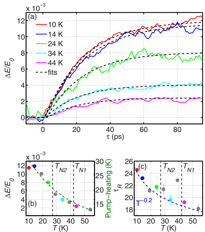
FIG. 4. (a) OPTP signals at different temperatures for t = 0 ps and F = 6 mJ/cm 2 . (b) Amplitude of the OPTP signals vs temperature. The right y axis shows the pump-induced heating (dashed line), calculated from the heat capacity and fluence [24]. (c) The rise time of the OPTP signals vs T , extracted from an exponential fit. The blue dashed line is a power-law fit, where the power Q = -0.2 . In both (b) and (c), the dashed lines show the transition temperatures T_{N1} and T_{N2} .
