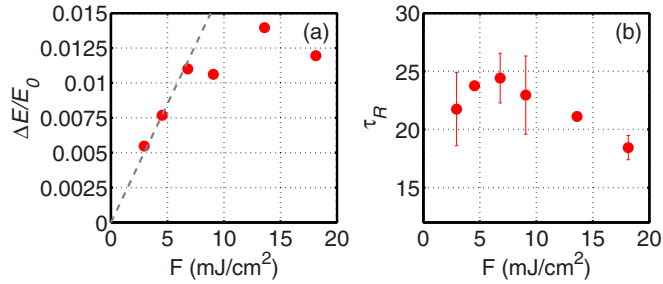
FIG. 5. (a) The amplitude and (b) time constant \tau_R extracted from OPTP signals measured at 10 K for different fluences and t = 0 ps. The dashed gray line in (a) illustrates the linear dependence of the amplitude on fluence up to 7 mJ/cm 2 .
