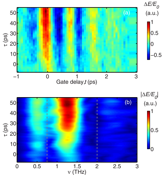
FIG. 3. (a) Photoinduced change in the transmitted THz pulse, \Delta E/E_0 , vs gate delay t and pump-probe delay \tau at T = 10 K. (b) The Fourier transform of (a), showing |\Delta E(v, \tau)/E_0| , i.e., the power spectrum vs \tau . The gray dashed lines at 0.75 and 2 THz show the positions of the electromagnons.
