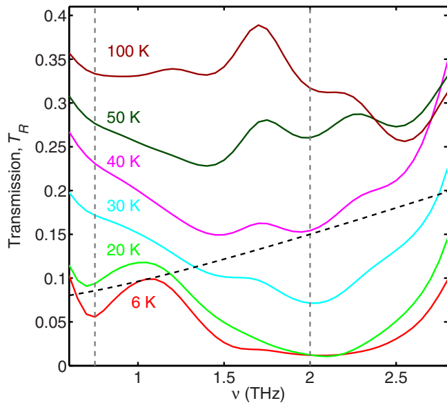
FIG. 1. THz transmission, T_R , vs frequency \nu (without optical photoexcitation) and sample temperature through a 150- \mu\text{m} -thick ac-oriented TbMnO 3 crystal, with the THz E -field polarized along the crystal a axis. T_R is defined as |E_{\text{trans}}(\nu)/E_{\text{in}}(\nu)| , where E_{\text{in}}(\nu) is the incident THz pulse and E_{\text{trans}}(\nu) is the transmitted pulse. The dashed gray lines indicate the positions of the electromagnon resonances. The dashed black line shows a calculated Drude response.
