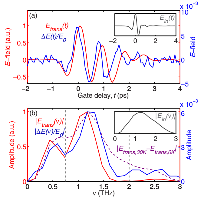
FIG. 2. (a) THz E field vs time transmitted through the crystal (red) [ E_{\text{trans}}(t) ] without photoexcitation, and the photoinduced change vs time in the THz E field (blue) given by \Delta E/E_0 = [E_{\text{pumped}}(t) - E_{\text{trans}}(t)]/E_0 and normalized to the maximum of E_{\text{trans}} , E_0 . These curves were measured at \tau = 100 ps. The inset shows the THz E field before the TbMnO 3 crystal, E_{\text{in}}(t) . (b) The spectra of the curves in Fig. 2(a). The purple dashed line simulates how the transmitted THz spectrum changes with 24 K of heating, calculated by Fourier transforming [E_{\text{trans}}(t) (30 \text{ K}) - E_{\text{trans}}(t) (6 \text{ K})] and taking the absolute value of the result. All other curves were measured at T \sim 6 K.
