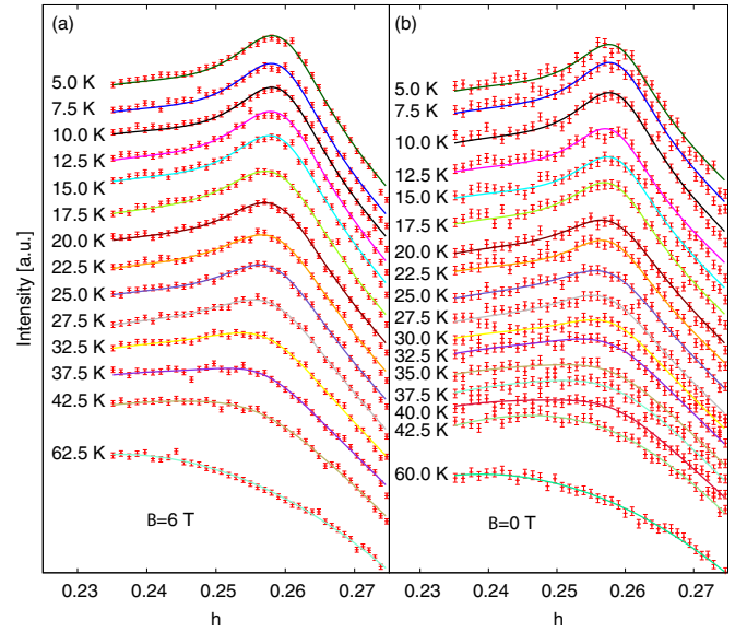
FIG. 2. RSXS (red bars) and Lorentzian fits on the electronic order peak for B = 6 (a) and 0 T (b). For each scan, \alpha , k , s , and h_0 from Eq. (1) were free fit parameters. \beta and \gamma were assumed to depend on the magnetic field, but not on temperature and taken from the RSXS scans at T = 60 K. For T > 42.5 K, reliable fits of the RSXS could not be achieved due to the strong correlation of fit parameters. The data for 62.5 K (60 K) were thus fitted with k in Eq. (1) set to zero. For B = 6 T (a), the RSXS signal of three consecutive, identical scans was summed up to achieve superior statistics, while for B = 0 T, the RSXS was only measured once for each temperature.
