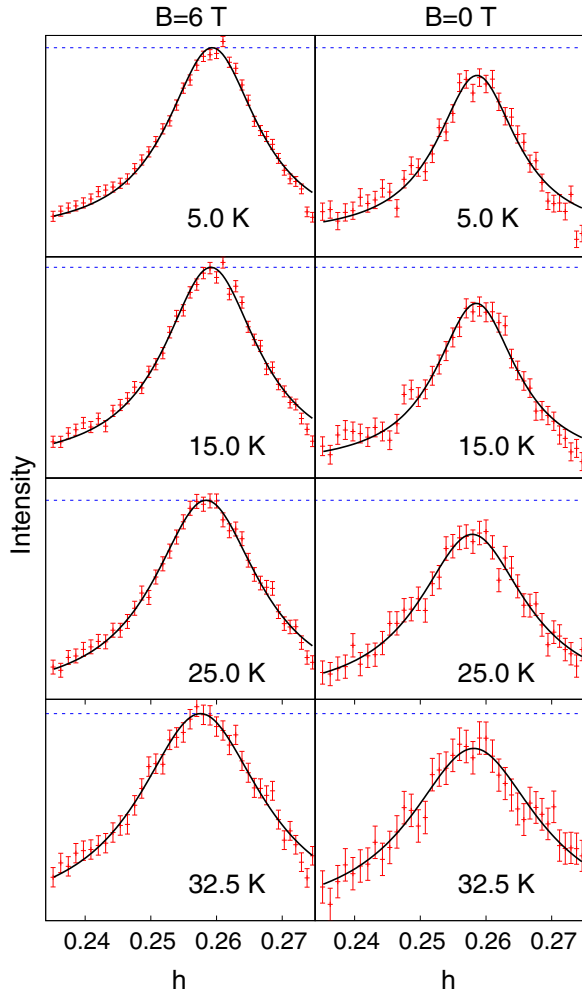
FIG. 4. Selected RSXS and Lorentzian fits on the electronic order peak for B = 6 and 0 T. Only the Lorentzian contribution from Eq. (1) is shown, while the background was subtracted from fits and experimental data. For each scan, \alpha , k , s , and h_0 from Eq. (1) were free fit parameters. \beta and \gamma were assumed to depend on the magnetic field, but not on temperature and taken from the RSXS scans at T = 60 K. For B = 6 T, the RSXS signal of three consecutive, identical scans was summed up to achieve superior statistics, while for B = 0 T, the RSXS was only measured once for each temperature. Blue dotted lines are a guide to the eye for the B = 6 T maximum intensity. For all measured temperatures, the superlattice peaks at 6 T are slightly more intense as compared to zero field.
