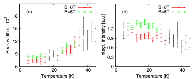
FIG. 3. (a) Peak width s from Lorentzian fits of the RSXS in Fig. 2. The electronic order peak is broader when a magnetic field is applied. The weak variation of the peak width with temperature is similar for both cases. (b) Integrated intensity of the electronic order peak at B = 0 (red) and 6 T (green), taken from Lorentzian fits with Eq. (1). The electronic order peak is more intense in a magnetic field and the transition temperature T_{\text{CO}} is increased.
