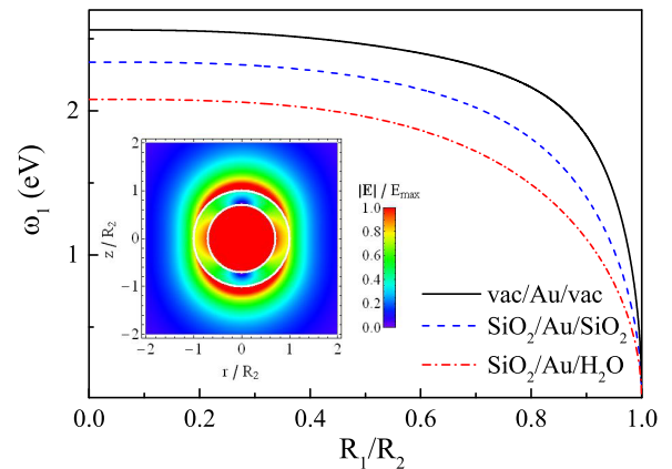
FIG. 1. Frequency of bright dipole plasmon mode in gold NS with various core and outside dielectrics is plotted vs NS aspect ratio. Inset: Electric field distribution for \text{SiO}_2/\text{Au}/\text{H}_2\text{O} NS with aspect ratio R_1/R_2 = 0.7 .
