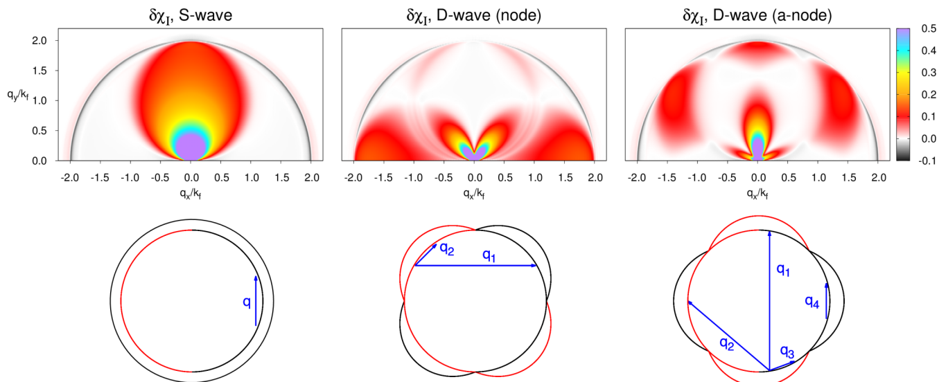
FIG. 2. Top panels show static susceptibility \delta\chi_I(0, \mathbf{q}, 0) as a function of ordering vector \mathbf{q} at the center of the domain wall in the limit of low field \mu_B H/\Delta_0 = 0.01 and temperature k_B T/\Delta_0 = 0.05 . The purple region around \mathbf{q} = 0 (uniform magnetization) has enhancement \delta\chi'_I > 0.5 due to large density of bound states and has been removed to better highlight the main features. The S -wave superconductor (left) favors \mathbf{q} \parallel \hat{y} , along the domain wall. A domain wall along nodes of D -wave superconductor (middle) increases tendency for AFM with q_x \sim 1.75k_f , across the domain wall. For antinodally oriented domain wall (right) enhancement of \chi shows for \mathbf{q}/k_f \sim (0, 2) and (1.25, 1) . Bottom panels show ordering vectors \mathbf{q} that connect points on the Fermi surface with same signs of \Delta_{\hat{k}f} and \Delta_{\hat{k}'f} that give largest coherence factors between zero-energy bound states. The OP at the final end of quasiclassical trajectory \hat{k} , \Delta_{\hat{k}f} , is a product of the domain wall spatial profile (inner circle) and the symmetry factor g_{\hat{k}} (outer profile). black/red denote signs \pm 1 .
