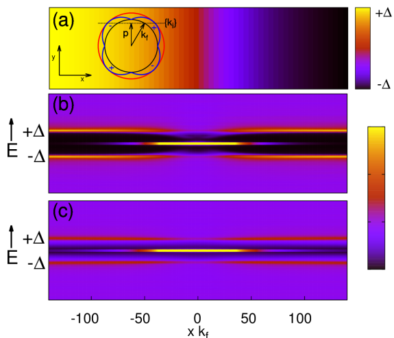
FIG. 1. (a) Domain wall +\Delta \rightarrow -\Delta in the x direction with translational invariance along y . Inset shows relative orientation of the domain wall plane and internal symmetry of the order parameter, S (red) or D -wave (blue). (b) The normalized local density of states N(\epsilon, x)/N_f for S -wave domain wall, and (c) the same for D -wave with nodes \parallel x . The zero-energy states appear at the domain wall. We use \Delta_0 = 0.05\epsilon_f throughout the paper that results in \xi_c k_f \sim 12 .
