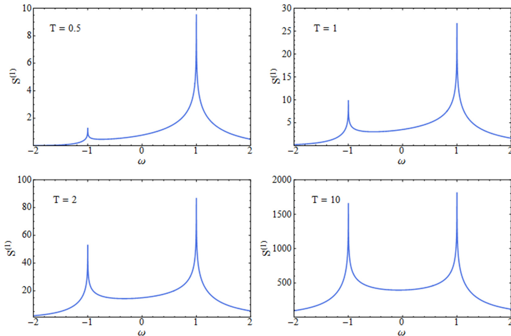
FIG. 3. The one-loop contribution to the longitudinal part of the dynamical structure factor for a ferromagnet, Eq. (2.21), normalized by \sqrt{\omega_k}/4\pi D^{3/2} , for H = 0 as a function of the frequency \omega for various values of the temperature T . \omega and T are measured in units of \omega_k . On the scale shown, the result for T/\omega_k = 10 is almost indistinguishable from the classical result, Eq. (2.22).
