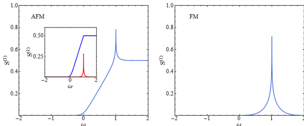
FIG. 5. The one-loop contribution to the longitudinal part of the dynamical structure factor for an antiferromagnet (left panel) and a ferromagnet (right panel), normalized by N_0^2 c / 4\pi\rho_s^2 and as in Figs. 4 and 3, respectively, for T/\omega_k = 0.05 as functions of the frequency \omega measured in units of \omega_k . The inset in the left panel separately shows the T = 0 contribution to the antiferromagnetic structure factor (blue curve) and the contribution that vanishes as T \rightarrow 0 (red curve). The structure factor shown in the main panel is the sum of these two, see Eq. (2.36).
