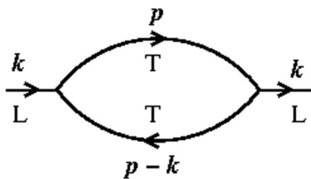
FIG. 1. Diagrammatic representation of the coupling between longitudinal and transverse spin fluctuations in the classical case: A longitudinal (L) mode couples to two transverse (T) modes. The resulting contribution to the longitudinal susceptibility \chi_L has the form given in Eq. (1.1).
