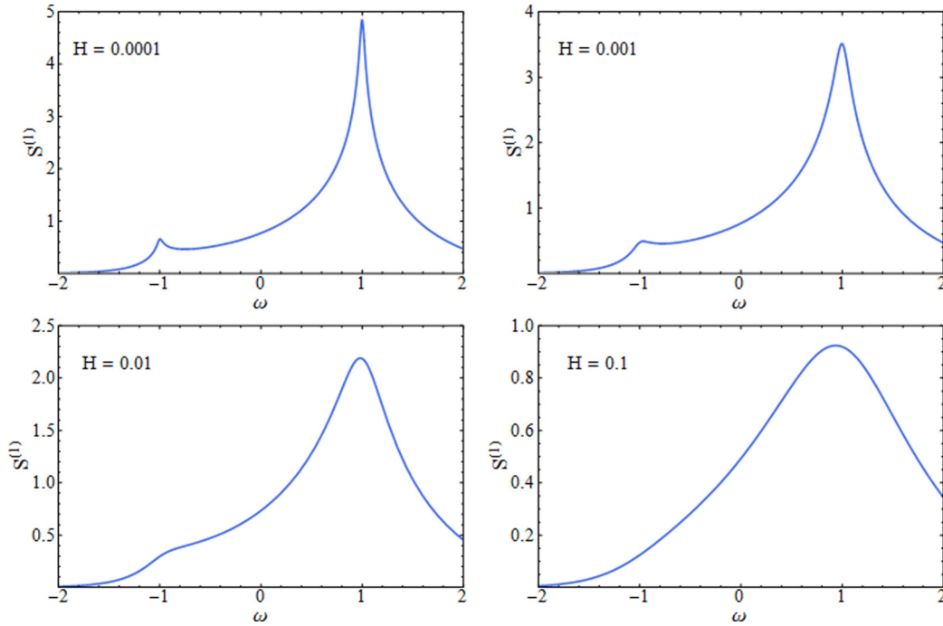
FIG. 4. The one-loop contribution to the longitudinal part of the dynamical structure factor for a ferromagnet, Eq. (2.21), normalized as in Fig. 3, for T/\omega_k = 0.5 as a function of the frequency \omega for various values of the magnetic field H . \omega and H are measured in units of \omega_k and \omega_k/\mu , respectively. Notice how even a very weak magnetic field broadens the resonance feature.
