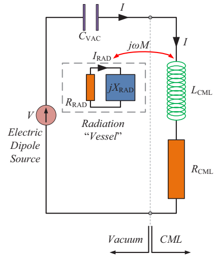
FIG. 4. Sketch of the equivalent circuit for excitation by a particular evanescent TM plane-wave component. The wave impedance of TM waves in vacuum Z_0 corresponds to the capacitance C_{\text{VAC}} , while the impedance Z of the CML contains a loss resistor R_{\text{CML}} and an inductive L_{\text{CML}} component. The cylindrical vessel in the near field of vacuum-CML interface is characterized by a radiation resistance R_{\text{RAD}} and a reactive impedance X_{\text{RAD}} .
