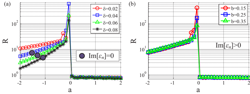
FIG. 5. The radiation enhancement ratio R as a function of the real part of the transversal components a = \text{Re}[\varepsilon_t] = \text{Re}[\mu_t] for (a) several perturbation parameters \delta = \text{Im}[1/\varepsilon_t - \varepsilon_n] of the normal component of the material parameters (with b = 0.1 ) and (b) several values of the imaginary part b = -\text{Im}[\varepsilon_t] = -\text{Im}[\mu_t] (with \delta = 0.03 ). Plot parameters: r = \lambda_0/200 , N = 80 , g = \lambda_0/20 , L = 3\lambda_0 , \theta = 90^\circ .
