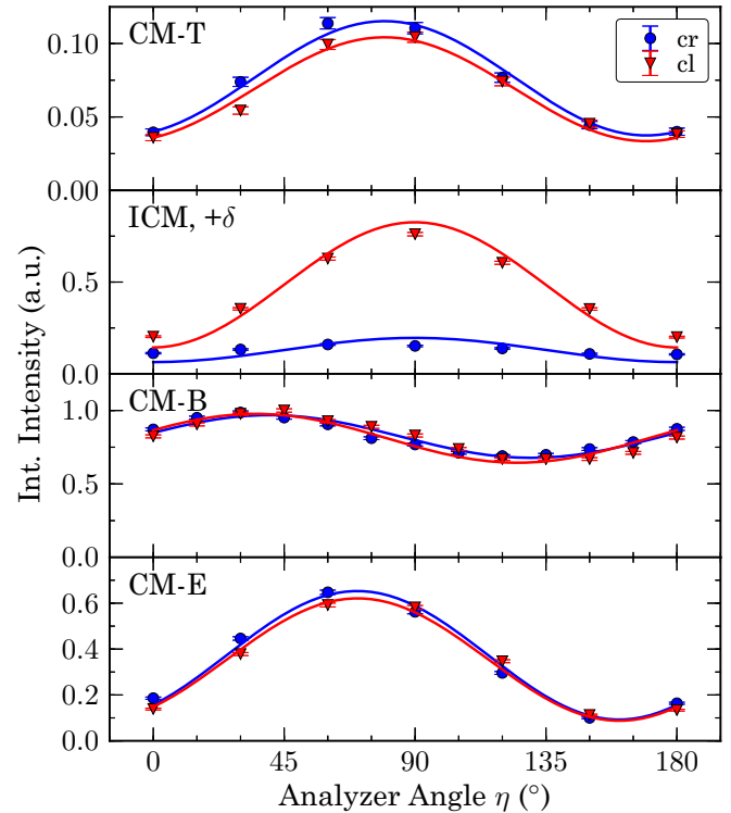
FIG. 5. Comparison of experimental (symbols) and simulated (lines) Stokes scans for circular right ( c_r ) and circular left ( c_l ) polarized incoming photons. The measured superlattice peaks are (0 0 7.5) and (0 0 7.5 + \delta ) for CM and ICM, respectively. Temperature and fields for the shown measurements are: CM-T: 20 K, no field. ICM: 5.8 K, no field. CM-B: 2 K, 2 T. CM-E: 5.8 K, 88 kV/m.
