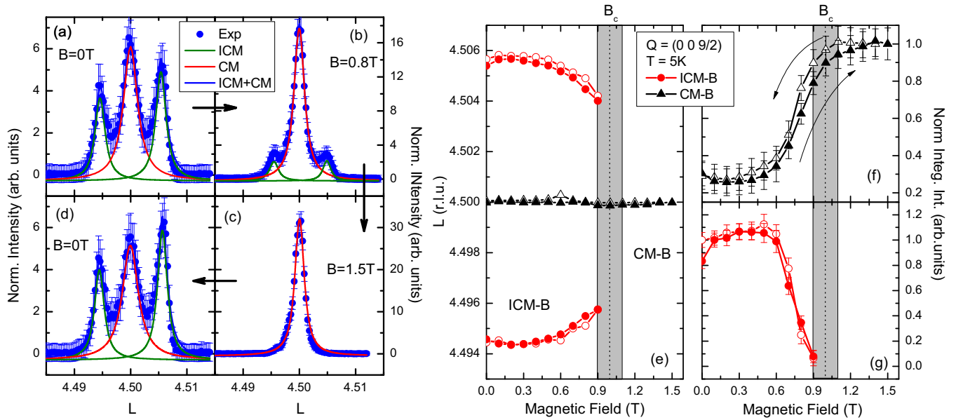
FIG. 3. Magnetic field dependence of magnetic satellite reflections around (0,0,4.5) at 5 K. (a)–(d): L scans through the (0,0,4.5) peak at various magnetic fields. The magnetic field induced changes closely correspond to the ones induced by electric fields (cf. Fig. 2). The solid lines represent again fits to the data. Extracted fit parameters as a function of applied magnetic field are presented in (e)–(g). Field loops up to 1.5 T and back to 0 T are shown. (e) Position of the CM and ICM peaks, (f) integrated intensity of the CM peak, and (g) total integrated intensity of the ICM satellites at \pm\delta . In none of the measurements a clear hysteresis appears. The critical field B_c is defined by the disappearance of the ICM satellites, where the shaded region indicates the uncertainty of our experiment.
