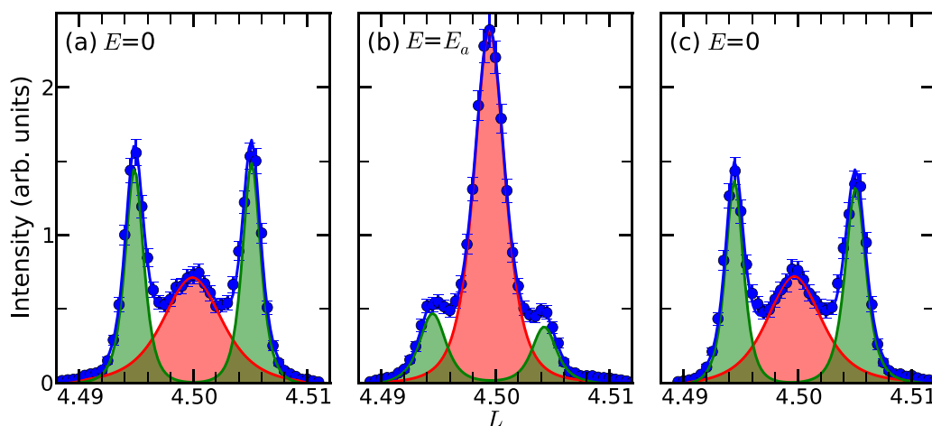
FIG. 2. E -field dependence of the L scans around the (0\ 0\ 4.5) position at 5.8 K, fitted by three Lorentzian squared functions plus a linear background. The separate peaks of the fit are shown as green and red lines, representing the ICM (green) and CM satellites (red). The sum of the fitted peaks and the linear background (blue line) agrees well with the experimental data (blue dots). (b) Upon applying a moderate electric field of E_a = 88 \text{ kV/m} , a dramatic change in the magnetic scattering is observed. (c) After removing E , the initial intensity profile is recovered, i.e., the process is reversible.
