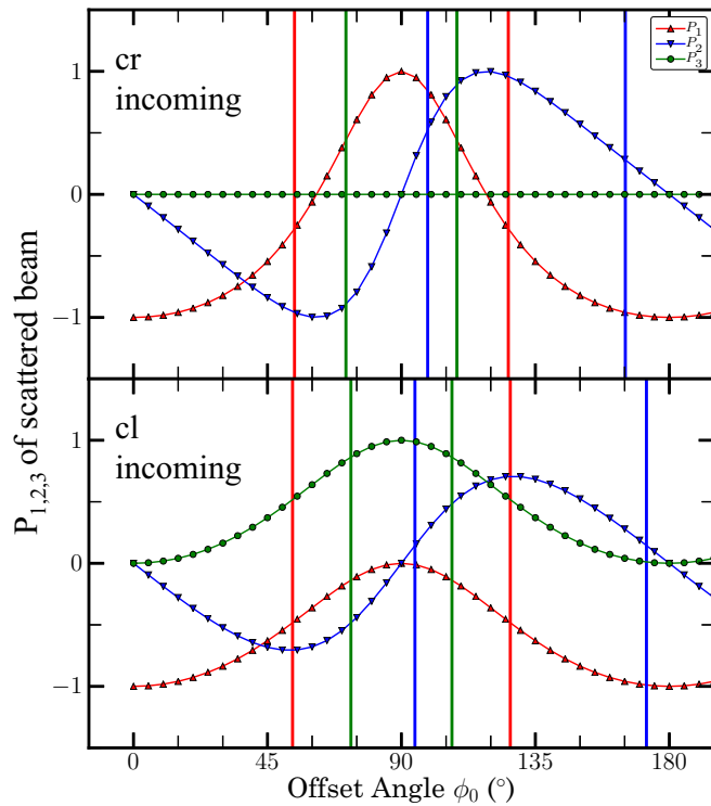
FIG. 6. Comparison of the calculated and observed P_{1,2,3} of the scattered beam for the (0,0,7.5) reflection at the Nd L_2 edge, measured with circular right (cr) and circular left (cl) polarized incoming light. The curves were calculated using a monodomain model by varying the value of \phi_0 . The vertical lines indicate the \phi_0 values at which the calculated P_{1,2,3} matches the corresponding experimental value.
