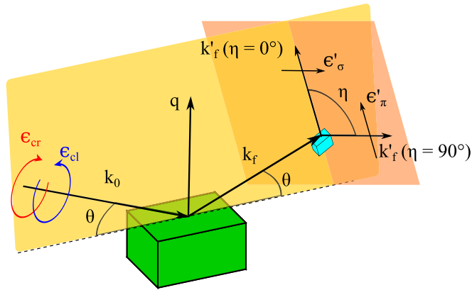
FIG. 4. Scattering geometry used during the Stokes analysis. The incoming photon with wave vector k_0 is circularly right ( \epsilon_{cr} ) or left ( \epsilon_{cl} ) polarized. The scattered beam with wave vector k_f is again diffracted by the analyzer crystal, shown in blue. The scattered x ray is linearly polarized \epsilon' . By rotating the analyzer crystal an angle \eta about the direction given by k_f , different components of the scattered beam polarization are selected, e.g., \epsilon'_\pi for \eta = 90^\circ and \epsilon'_\sigma for \eta = 0^\circ . \mathbf{q} is the scattering vector and \theta the Bragg angle.
