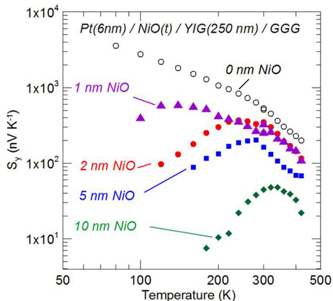
FIG. 2. Temperature dependence of the SSE signal on the Pt/YIG bilayer is compared to SSE signals from the YIG/NiO/Pt trilayers, with the NiO film thickness as noted. A decrease in SSE signal is observed with increasing NiO film thickness. A maximum at a temperature T_M is observed for each of the YIG/NiO/Pt trilayers. T_M increases with increasing NiO thickness.
