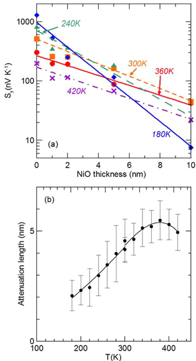
FIG. 3. (a) Magnitude of the SSE signal at 420, 360, 300, 240, and 180 K plotted as a function of NiO thickness. The experimental values are the data points. The lines through them are fitted exponential decay functions, with a characteristic attenuation length scale given as a function of temperature in (b).
