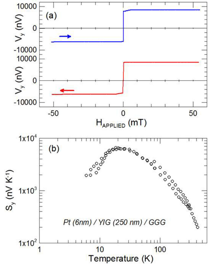
FIG. 1. (a) A raw trace of the spin Seebeck voltage V_y vs applied field at 300\text{ K} for an applied heater power of 0.495\text{ W} and (b) spin Seebeck coefficient as a function of temperature for a Pt(6 nm)/YIG(250 nm) bilayer deposited on GGG \langle 111 \rangle . In (b), the results of several different runs in different instruments are superimposed on each other, illustrating the reproducibility of the results, which is of the order of 30\% . A maximum spin Seebeck coefficient of \sim 6.5 \pm 0.5\ \mu\text{V}/\text{K} is observed on the YIG film within a broad peak around 20\text{ K} .
