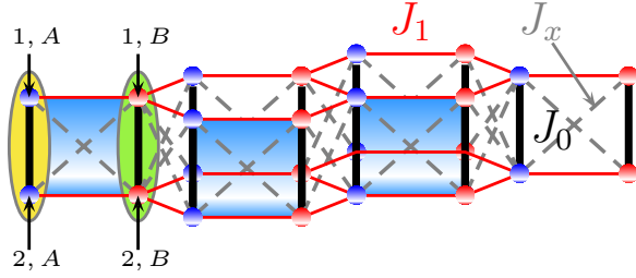
FIG. 1. Dominant exchange interactions in \text{Bi}_3\text{Mn}_4\text{O}_{12}(\text{NO}_3) . Colored areas correspond to the unit cells. Frustrating intralayer next nearest-neighbors interactions are omitted in this figure for simplicity.
