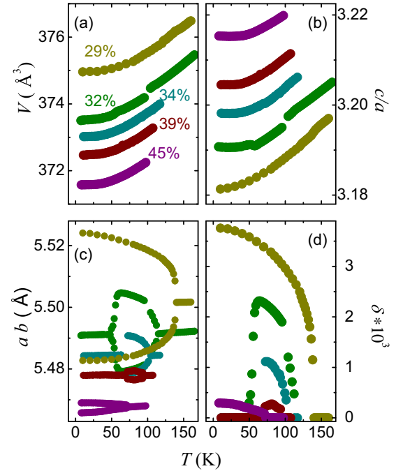
FIG. 3. Temperature dependence for the (a) volume ( V ), (b) lattice anisotropy, (c) a and b lattice parameters, and (d) orthorhombic order parameter ( \delta ) for compositions x = 0.29, 0.32, 0.34, 0.39 , and 0.45 determined from Rietveld refinements using synchrotron x-ray and spallation source neutron data.
