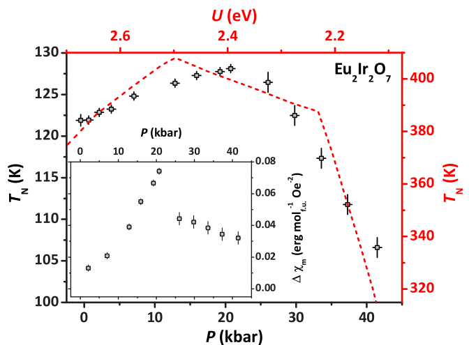
FIG. 6. Main panel: P dependence of the critical transition temperature (squares, bottom and left scales). The red dashed line (top and right scales) is obtained by digitizing data of the calculated EPD discussed in Ref. [24]. The right scale has been rescaled so that the scale zero coincides with that of the left scale. Inset: P dependence of the FC susceptibility \Delta\chi_m in the magnetic phase.
