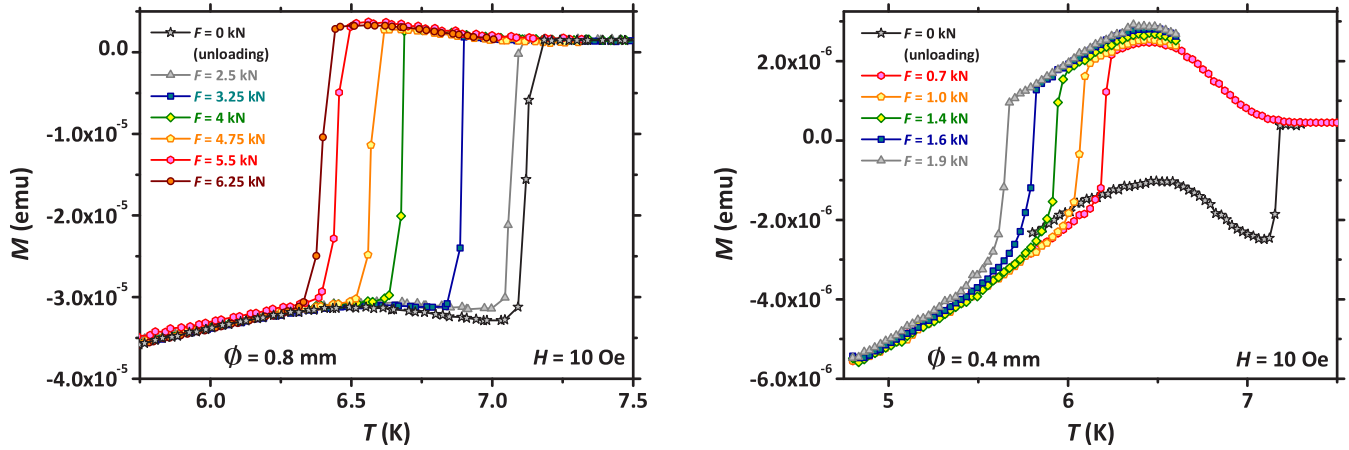
FIG. 2. Superconducting transitions of the Pb manometer for the gaskets with sample chamber diameter \varnothing = 0.8 mm (left panel) and \varnothing = 0.4 mm (right panel). The different curves correspond to different applied forces (see legend). The sudden jump in magnetization is ascribed to the diamagnetic contribution from the superconducting phase and its overall width is safely below 0.1 K for all the applied forces, denoting a good pressure homogeneity within the whole accessed experimental P range. The actual P values were quantified from Eq. (1). The other source of T dependence for M is the background signal from the PC, different for the two employed setups.
