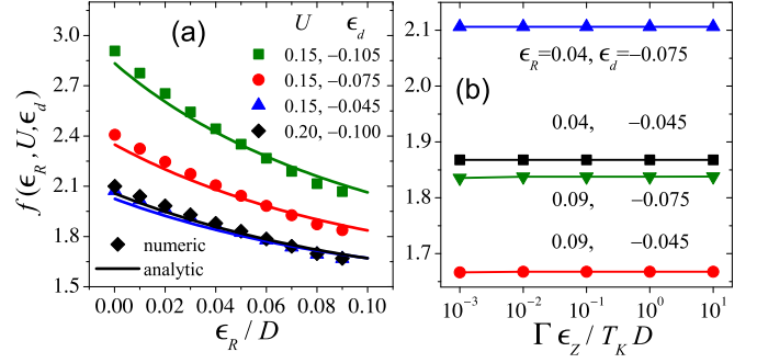
FIG. 9. Quantity f entering the scaling collapse of the impurity polarization for a system with fixed Fermi energy \epsilon_F = 0 : (a) f vs \epsilon_R for different values of U and \epsilon_d expressed in the legend in units of D . Each symbol was obtained via an NRG calculation of the compensating local field for \Gamma\epsilon_Z/T_K D = 0.1 , while the lines represent algebraic results based on Eq. (50). (b) NRG values of f vs \Gamma\epsilon_Z/T_K D for U = 0.15D and different values of \epsilon_R and \epsilon_d expressed in the legend in units of D . Lines are guides to the eye showing that f is independent of \epsilon_Z for \Gamma\epsilon_Z/T_K D \lesssim 10 . Data in both panels are for \epsilon_0 = -0.08D and \Gamma = 0.005D .
