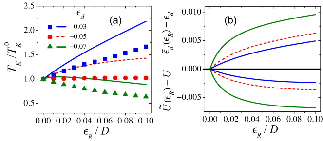
FIG. 5. (a) Scaled Kondo temperature T_K/T_K^0 vs Rashba energy \epsilon_R for fixed Fermi energy \epsilon_F = 0 and for different values of \epsilon_d expressed in the legend in units of D . Symbols represent NRG data and lines are the result of the perturbative treatment described in the text. (b) Perturbative shifts \tilde{\epsilon}_d - \epsilon_d and \tilde{U} - U in the effective impurity parameters vs \epsilon_R for the same cases shown in (a). Data are for \epsilon_0 = -0.08D , U = 0.1D , and \Gamma = 0.005D .
