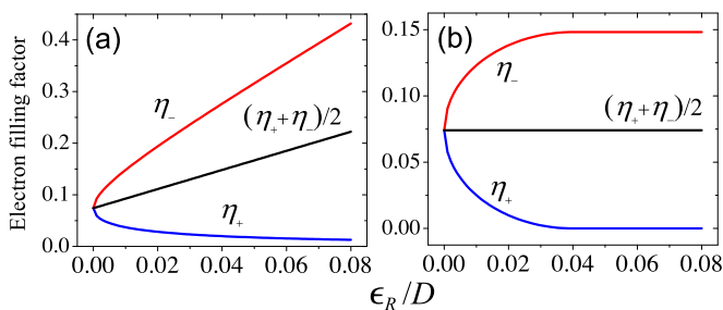
FIG. 2. Helicity-resolved conduction-band filling fractions \eta_{\pm} and overall filling fraction \eta = (\eta_+ + \eta_-)/2 , plotted as functions of Rashba energy \epsilon_R for \epsilon_0 = -0.08D and (a) fixed Fermi energy \epsilon_F = 0 , (b) constant filling fraction \eta = -\epsilon_0/(D - \epsilon_0) \approx 0.074 .
