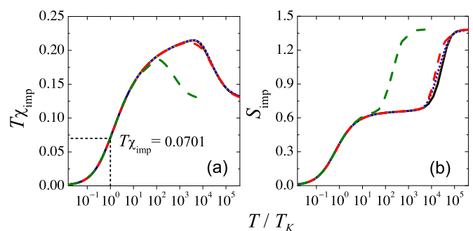
FIG. 4. Impurity contribution to (a) temperature times magnetic susceptibility T\chi_{\text{imp}} , and (b) entropy S_{\text{imp}} , both plotted vs scaled temperature T/T_K for five different cases: a no-Rashba reference (black solid line), and Rashba energies \epsilon_R/D = 0.04 (red and orange curves) and 0.08 (green and blue curves) under the scenarios of fixed Fermi energy (dotted lines) and constant band filling (dashed lines). The two dotted lines lie directly on top of one another on the scale of this plot. The Kondo temperature T_K is as defined in Eq. (44). Data are for \epsilon_0 = -0.08D , U = -2\epsilon_d = 0.1D , and \Gamma = 0.005D .
