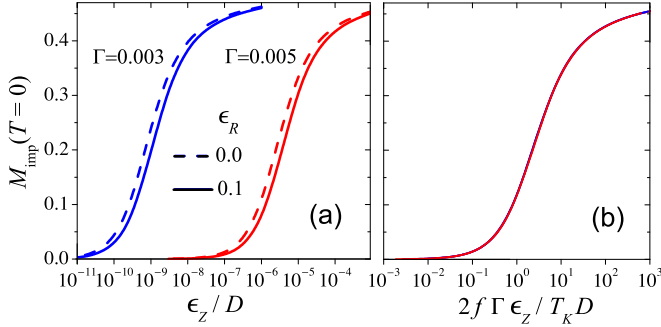
FIG. 8. (a) Zero-temperature impurity polarization M_{\text{imp}} vs Zeeman energy \epsilon_Z for a system with fixed Fermi energy \epsilon_F = 0 . Data are for \epsilon_0 = -0.08D , U = -2\epsilon_d = 0.15D , and the values of \Gamma and \epsilon_R labeled on the plot in units of D . (b) Same data as in (a), replotted vs 2f\Gamma\epsilon_Z/T_K D , where f = 2.4 and 1.8 for \epsilon_R/D = 0 and 0.1 , respectively.
