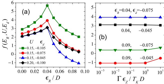
FIG. 11. Quantity f entering the scaling collapse of the impurity polarization for a system with constant band filling \eta \simeq 0.074 : (a) f vs \epsilon_R for different values of U and \epsilon_d expressed in the legend in units of D . Each symbol was obtained via an NRG calculation of the compensating local field for \Gamma \epsilon_Z/T_K D = 0.1 , while the lines are guides to the eye. (b) NRG values of f vs \Gamma \epsilon_Z/T_K D for U = 0.15D and different values of \epsilon_R and \epsilon_d expressed in the legend in units of D . Lines are guides to the eye showing that f is independent of \epsilon_Z for \Gamma \epsilon_Z/T_K D \lesssim 10 . Data in both panels are for \epsilon_0 = -0.08D and \Gamma = 0.005D .
