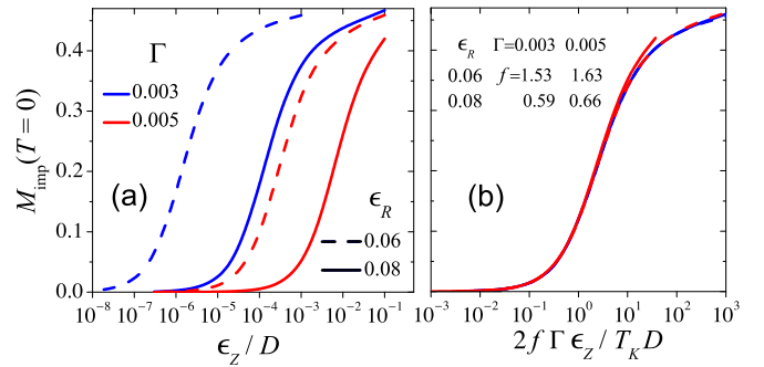
FIG. 10. (a) Zero-temperature impurity polarization M_{\text{imp}} vs Zeeman energy \epsilon_Z for constant band filling \eta \simeq 0.074 . Data are for \epsilon_0 = -0.08D , U = -2\epsilon_d = 0.15D , and the values of \Gamma and \epsilon_R labeled on the plot in units of D . (b) Same data as in (a), replotted vs 2f\Gamma\epsilon_Z/T_K D with values of f shown in the legend. In this case, f depends on \Gamma as well as \epsilon_R .
