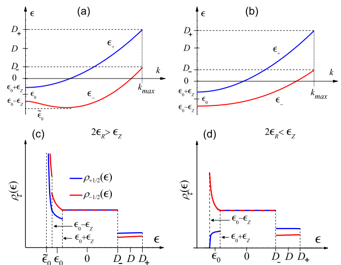
FIG. 3. Schematic plots of the effective angular-momentum-resolved densities of states \rho_t(\epsilon) obtained from Eq. (43) for (a) weak Zeeman splitting \epsilon_Z < 2\epsilon_R , (b) strong Zeeman splitting \epsilon_Z > 2\epsilon_R . In both panels, \rho_t(\epsilon) is constant and equal to its no-Rashba value \rho_0(\epsilon) throughout the energy range \epsilon_0 + \epsilon_Z < \epsilon < D_- .
