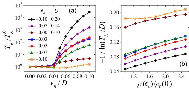
FIG. 6. Kondo temperature for a constant band-filling fraction \eta \simeq 0.074 : (a) T_K/T_K^0 vs \epsilon_R for different values of \epsilon_d and U expressed in the legend in units of D ; (b) results for \epsilon_R \geq 0.04D plotted as -1/\ln(T_K/D) vs \rho[\epsilon_F]/\rho_0(0) . Data are for \epsilon_0 = -0.08D and \Gamma = 0.005D .
