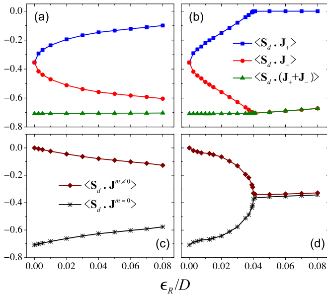
FIG. 7. Static correlations between the impurity spin and the total angular momentum in different conduction-band channels, calculated for (a), (c) fixed Fermi energy \epsilon_R = 0 , or (b), (d) constant band filling \eta \approx 0.074 . The upper panels show \langle \mathbf{S}_d \cdot \mathbf{J}_h \rangle for helicity h = \pm , while the lower panels plot the correlation of \mathbf{S}_d with \mathbf{J}^{m=0} (the total angular momentum of all electrons with orbital angular momentum m = 0 ) and with \mathbf{J}^{m \neq 0} defined in Eq. (49). Data are for \epsilon_0 = -0.08D , U = -2\epsilon_d = 0.1D , and \Gamma = 0.005D .
