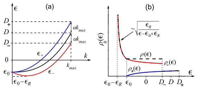
FIG. 1. Schematic plots of (a) the dispersion relations \epsilon_h(k) and (b) the densities of states per helicity channel \rho_h(\epsilon) , in the presence of Rashba SO interaction. The middle curve in (a) represents the dispersion \epsilon(k) in the absence of Rashba interaction. In (b), the combined density of states \rho(\epsilon) (dashed line) is constant and equal to its no-Rashba value \rho_0(\epsilon) throughout the energy range \epsilon_0 < \epsilon < D .
