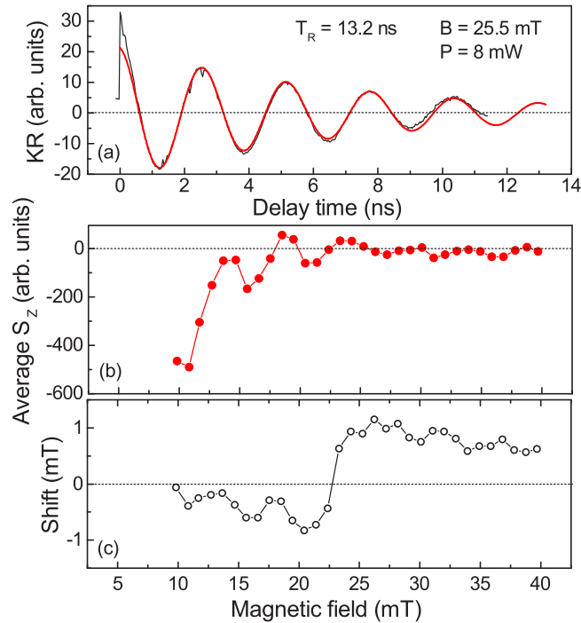
FIG. 5. (Color online) (a) Example of a time-resolved pump-probe Kerr signal measured at B = 25.5 mT (black curve). Red curve is a fit to the data with an exponentially decaying cosine function recorded over the full range of delays of T_R = 13.2 ns between two pump pulses. (b) Average electron spin polarization along the z axis resulting from the fitted curves as a function of magnetic field. (c) Reproduction of the data from Fig. 2(b) for simplified comparison with the data in panel (b).
