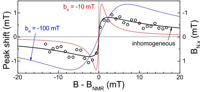
FIG. 9. (Color online) Peak shift and corresponding B_{N,x} calculated for the ^{77}\text{Se} isotope after Eq. (5) (black line) with b_e = -370 mT, S = 0.07 , and a_l = 3.4 nm. For comparison we show two homogeneously broadened curves calculated after Eq. (3) using b_e = -10 mT (red line) and b_e = -100 mT (blue line). Open circles represent the experimental data as in Fig. 2(b), but shifted slightly downwards to compensate for the offset.
