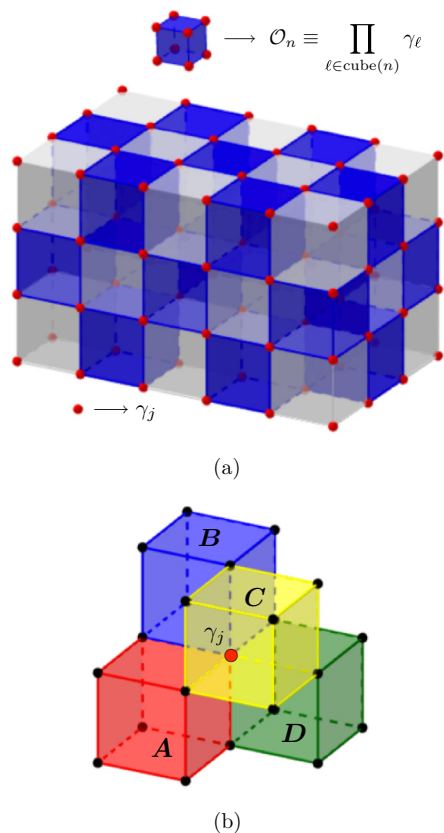
FIG. 1. (Color online) Majorana cubic model. The Majorana cubic model is defined on a cubic lattice, as in (a), with a single Majorana fermion per lattice site (colored red). The operator \mathcal{O}_n is the product of the 8 Majorana fermions at the vertices of a cube. The Hamiltonian is a sum of these local operators over every other cube (colored blue in (a)) in a checkerboard pattern. As any pair of operators either share exactly one edge or none, all operators mutually commute. We choose to label the cubic operators A, B, C , and D as shown in (b). Acting with a single Majorana operator \gamma_j at the indicated site creates these four excitations.
