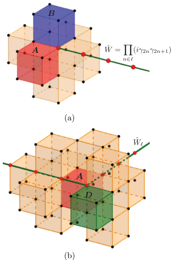
FIG. 2. (Color online) Dimension-1 particle. Excitations (colored) may be created by acting with Wilson line operators. In (a), a straight Wilson line creates pairs of dimension-1 particles at the end points. The dimension-1 particle may hop freely in the direction of the Wilson line, by acting with Majorana bilinear terms. Remarkably, the dimension-1 particle cannot hop in any other direction without creating additional excitations. Introducing a “corner” in the Wilson line, as in (b), creates an additional topological excitation localized at the corner.
