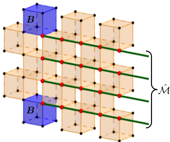
FIG. 4. (Color online) Membrane operator and fracton excitations. Acting with a product of Majorana operators on a surface \Sigma creates localized excitations at the corners of the boundary \partial\Sigma as shown above.
