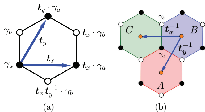
FIG. 5. (Color online) The Majorana plaquette model, as studied in [12]. Consider a honeycomb lattice with a single Majorana fermion on each lattice site. We define an operator \mathcal{O}_p as the product of the six Majorana fermions on the vertices of a hexagonal plaquette p , as shown in (a). The colored plaquettes in (b) correspond to the three distinct bosonic excitations with mutual semion statistics ( A , B , or C ) that may each be created in pairs by acting with Wilson line operators.
