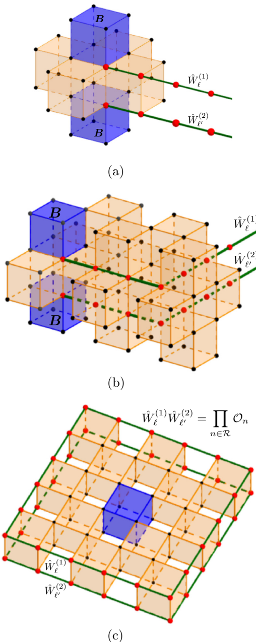
FIG. 3. (Color online) Dimension-2 anyon. Acting with two adjacent Wilson line operators \hat{W}_1 and \hat{W}_2 creates pairs of excitations at the end points of the same type ( AA, BB, CC , or DD ). These two-fracton excitations are free to move in a two-dimensional plane orthogonal to the shortest line segment connecting the pair of Wilson lines. Furthermore, in (b) we may detect a fracton (colored blue) by braiding a dimension-2 anyon around a closed loop enclosing the fracton. As the braiding operator, a pair of closed Wilson line operators \hat{W}_1 \hat{W}_2 is equal to the product of the enclosed cube operators as shown above. Therefore, the braiding produces an overall minus sign if an odd number of fractons are enclosed.
