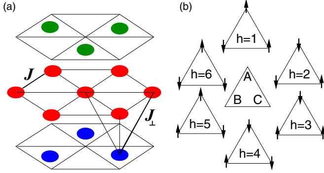
FIG. 1. (Color online) (a) The multilayer triangular lattice with abc stacking. (b) The mapping (modulo 6) from ground-state spin configurations on sublattices A, B, and C to integer-valued height variables h (adapted from Ref. [11]).
