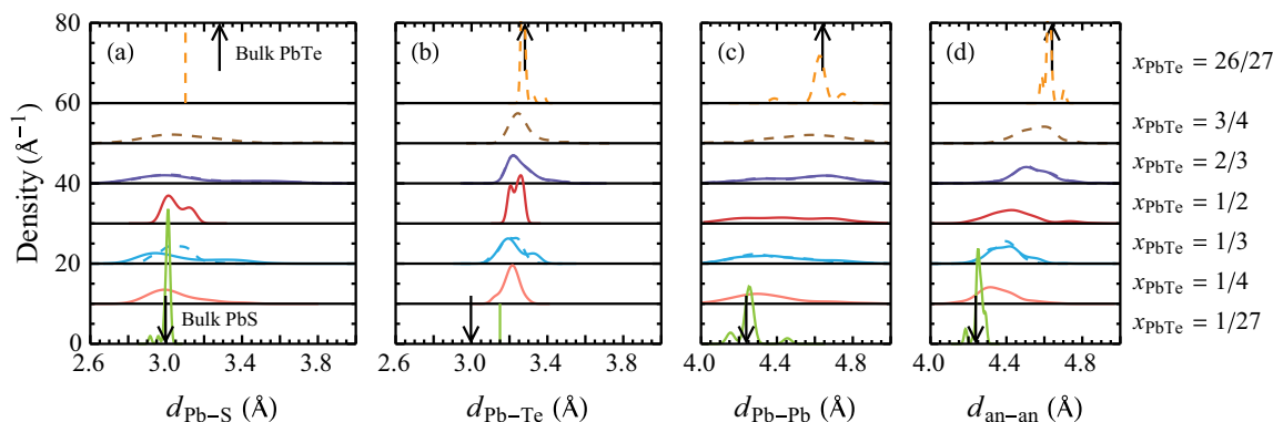
FIG. 6. (Color online) Distribution of bond lengths in PbS-PbTe SQS. Bond lengths shown are 1NN (a) Pb-S ( d_{\text{Pb-S}} ) and (b) Pb-Te ( d_{\text{Pb-Te}} ) bonds, and 2NN (c) Pb-Pb ( d_{\text{Pb-Pb}} ) and (d) anion-anion ( d_{\text{an-an}} ) bonds. Bond-length distributions of SQS in their energy minima are shown as solid lines and bond-length distributions of SQS at saddle points in their energy landscapes are shown as dashed lines. Arrows indicate the corresponding bond lengths in bulk PbS and PbTe. Distributions are offset along the y axis for clarity (with corresponding x axes shows as horizontal dashed lines).
