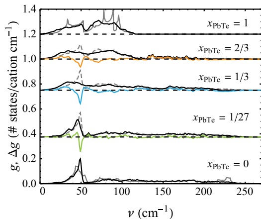
FIG. 2. (Color online) Phonon DOS of mixing for PbS-PbTe SQS. Total phonon DOSs ( g ) for each SQS are shown as solid black lines. Composition-weighted averages of the phonon DOS of PbS and PbTe [ xg_{\text{PbTe}} + (1-x)g_{\text{PbS}} ] are shown as dashed gray lines. The difference between these curves, the phonon DOS of mixing ( \Delta g ), defined in Eq. (11), are shown as solid colored lines for 54-atom SQS with stable phonon modes. Phonon DOSs derived from experimental neutron-diffraction data for PbS [82] and PbTe [81] are shown as solid gray lines. Each phonon DOS is offset along the vertical axis for clarity; dashed lines indicate the zero for each phonon DOS.
