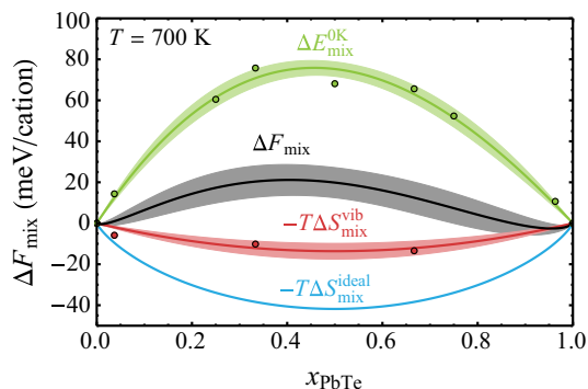
FIG. 3. (Color online) Contributions to the free energy of mixing \Delta F_{\text{mix}} [Eq. (4)] at 700 K: 0 K mixing energetics \Delta E_{\text{mix}}^{\text{OK}} (green), vibrational entropy of mixing -T\Delta S_{\text{mix}}^{\text{vib}} (red), and ideal entropy of mixing -T\Delta S_{\text{mix}}^{\text{ideal}} (blue). Green data points and solid line show DFT-calculated energetics and a subregular solution model fit to this data, respectively. Red data points and solid line show vibrational entropies of mixing calculated from \Delta g(\nu) and a regular solution model fit to this data, respectively. Shaded regions show 90% confidence intervals for fits to \Delta E_{\text{mix}}^{\text{OK}} , \Delta S_{\text{mix}}^{\text{vib}} , and their summed contribution to \Delta F_{\text{mix}} .
