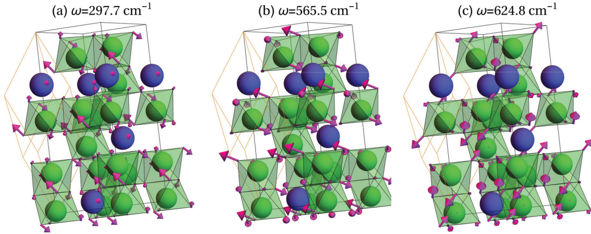
FIG. 3. (Color online) Displacement patterns for the three characteristic phonons that display large spin-lattice coupling across the Néel transition. Ni and Te ions are shown in green and blue, respectively; oxygens (not drawn) are at octahedral vertices. Ionic displacements are indicated by pink arrows whose length is proportional to the displacement. The rhombohedral unit cell, indicated by the orange lines, contains one \text{Ni}_3\text{TeO}_6 formula unit.
