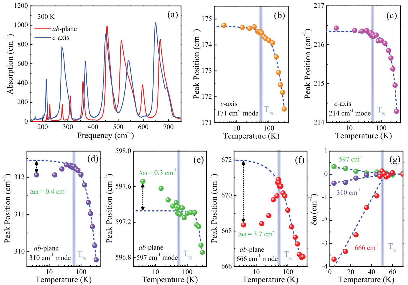
FIG. 2. (Color online) (a) Polarized infrared absorption spectrum of \text{Ni}_3\text{TeO}_6 at 300 K. (b)–(f) Peak position vs temperature for several characteristic phonons. A Boltzmann sigmoid fit was used to model anharmonic and short range order effects, and the difference between the low temperature limit of this model (which gives the unperturbed frequency) and the phonon position at base temperature was used to extract the frequency shifts ( \delta\omega 's). The Néel temperature is indicated by a vertical line at 53 K. (g) Spin-lattice coupling-induced frequency shifts, \delta\omega 's, for the three ab -plane phonon modes from panels (d)–(f), now plotted on a linear temperature scale, together with linear fits to the model described in the text.
