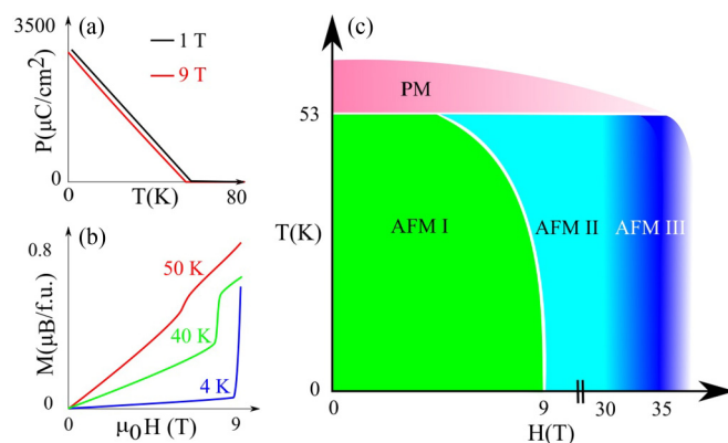
FIG. 1. (Color online) (a) Temperature dependence of the electric polarization P_c(H_c) showing the magnetically induced polarization change below the 53 K Néel transition [1]. (b) Magnetization curves at different temperatures [1]. (c) Schematic phase diagram of \text{Ni}_3\text{TeO}_6 for H \parallel c showing the 9 T spin flop and the possibility of an unexplored transition between 30 and 35 T.
