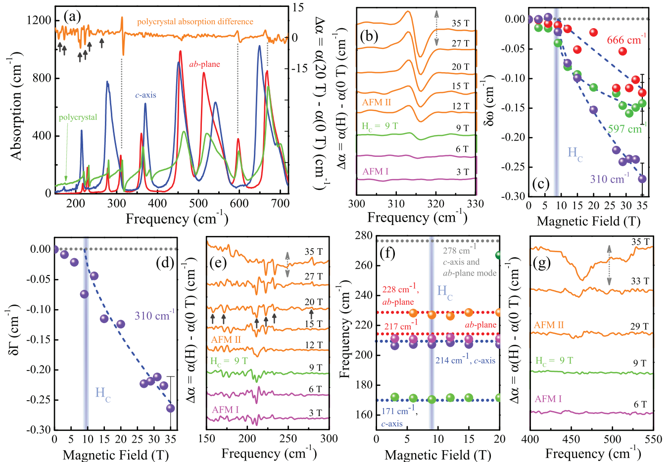
FIG. 4. (Color online) (a) Polarized infrared absorption spectrum, the polycrystal response, and the absorption difference spectrum at 20 T. The latter highlights the changes in the elastic properties between the AFM-I and AFM-II phases and is defined as \Delta\alpha = \alpha(\omega, H) - \alpha(\omega, H = 0) . (b)–(d) Close-up view of the field-induced absorption difference spectrum in the vicinity of the 310 cm -1 mode through the 9 T spin-flop transition along with the field-induced frequency shift and linewidth changes. The curves in (b) are offset for clarity, and the dotted arrow is a 20 cm -1 scale bar. The vertical line in (c) and (d) indicates the 9 T critical field. (e), (f) Close-up view of the field-induced absorption difference spectra in the vicinity of the most collective vibrational modes along with a contour plot revealing the subtle frequency shifts through the spin-flop transition. The curves in (e) are offset for clarity, and a 20 cm -1 scale bar is included. (g) Waterfall plot in the vicinity of the 451 and 456 cm -1 modes providing evidence for an unexplored transition between 30 and 35 T. Each curve in the waterfall plot is offset for clarity, and a scale bar is 20 cm -1 . All data was taken at 4.2 K.
