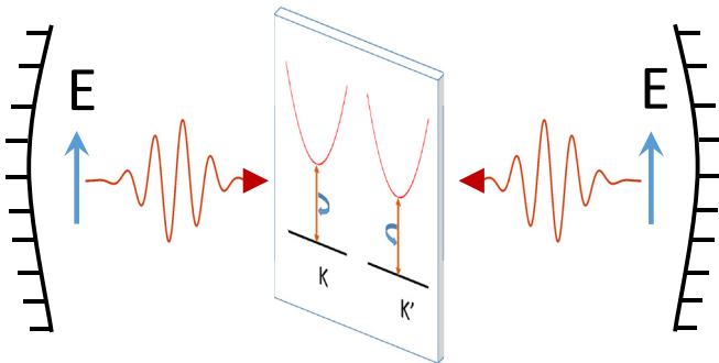
FIG. 2. (Color online) Valley entanglement of excitons in K and K' valleys of an \text{MX}_2 monolayer in a cavity geometry.
