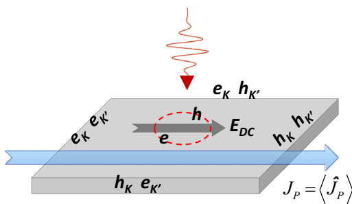
FIG. 3. (Color online) A sketch of photocurrent detection. Under illumination with a linearly polarized single-photon field and in the presence of an in-plane dc electric field E_{DC} there is charge separation in the direction along E_{DC} which gives rise to a photocurrent J_P if a monolayer is contacted and included in a proper external circuit. There is no photocurrent or photovoltage in the transverse direction.
