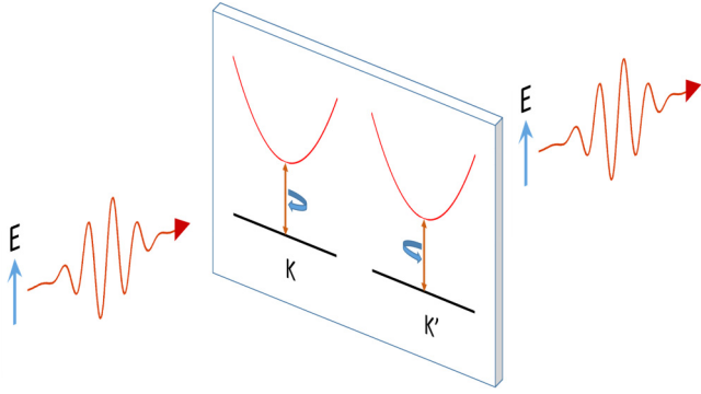
FIG. 1. (Color online) A sketch of excitons in K and K' valleys of \text{MX}_2 monolayers interacting with linearly polarized single photons. To ensure the interaction with one photon at a time, the power of incident radiation should not exceed \hbar\omega\Delta\omega , where \Delta\omega is the radiation bandwidth.
