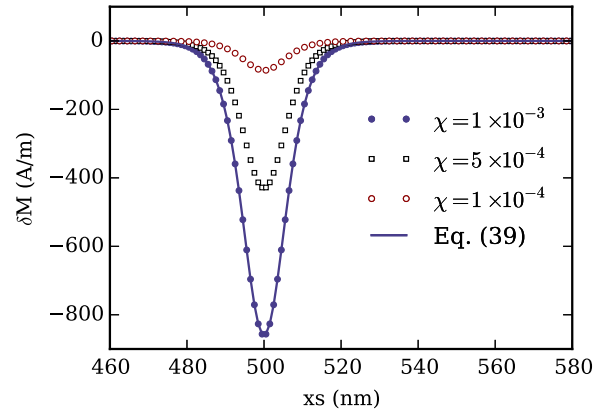
FIG. 5. (Color online) Simulation results of the magnetization length difference \delta M for a 1D domain wall located at x = 500 nm with M_e = 8.6 \times 10^5 A/m and A = 1.3 \times 10^{-11} J/m. The demagnetization factors are selected to be N_x = 0 and N_y = N_z = 0.5 .
