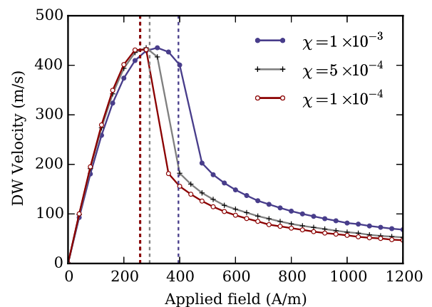
FIG. 4. (Color online) Simulation results of domain-wall velocities for various susceptibilities. The parameters used are \alpha = 0.001 , \beta = 0 , N_y = 0.2 , and N_z = 0.8 . The vertical dashed lines are the breakdown fields computed using Eq. (53).
