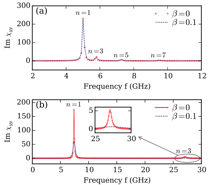
FIG. 3. (Color online) Imaginary parts of the dynamical susceptibility \chi_{yy} of the film for (a) thickness d = 300 \text{ nm} and (b) thickness d = 60 \text{ nm} .
