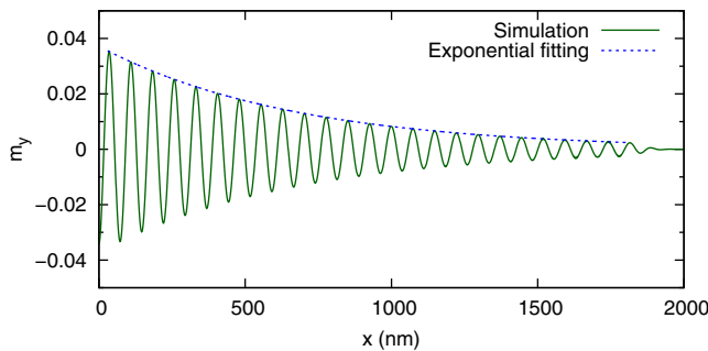
FIG. 1. (Color online) The spin-wave-amplitude decay along the rod, for a spin wave excited locally by applying a microwave \mathbf{H} = H_0 \sin(2\pi f t) \mathbf{e}_y , of frequency f = 30 GHz and amplitude H_0 = 1000 Oe in the region 0 \leq x \leq 2 nm. The data were fitted using Eq. (23) with \beta = 0.02 and \alpha = 0.01 .
