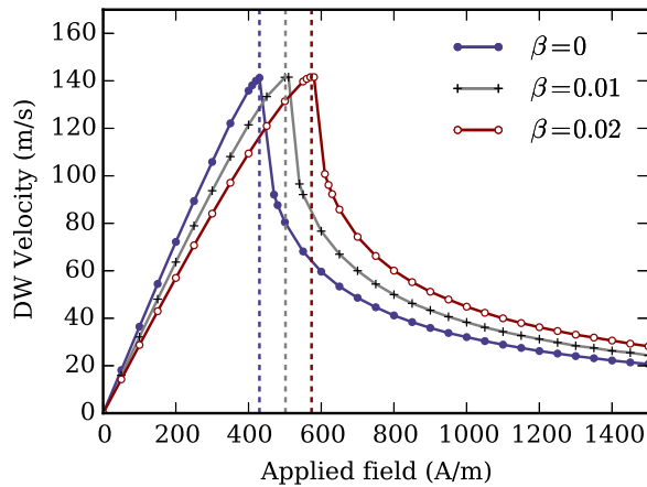
FIG. 6. (Color online) Simulation results of domain-wall velocities for the limit case that \chi \rightarrow 0 with various exchange dampings. The parameters used are \alpha = 0.005 , N_y = 0.4 , and N_z = 0.6 . The vertical dashed lines are the breakdown fields computed with Eq. (60).
