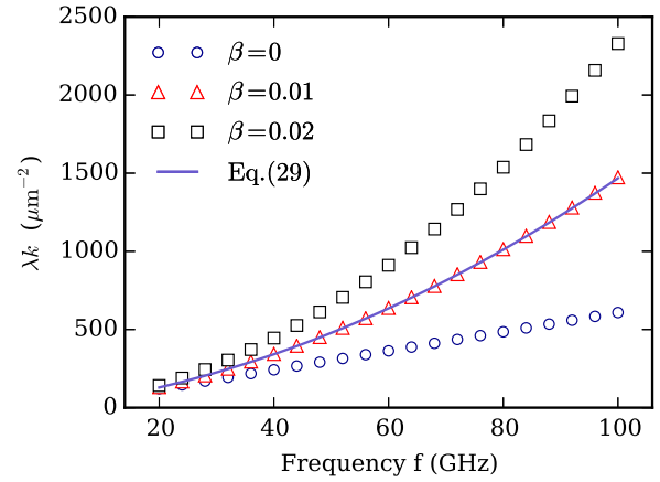
FIG. 2. (Color online) The spin-wave-decay constant-wave vector product \lambda k as a function of the frequency for different \beta values. The slate blue line was drawn using Eq. (29) for the case \beta = 0.01 .
