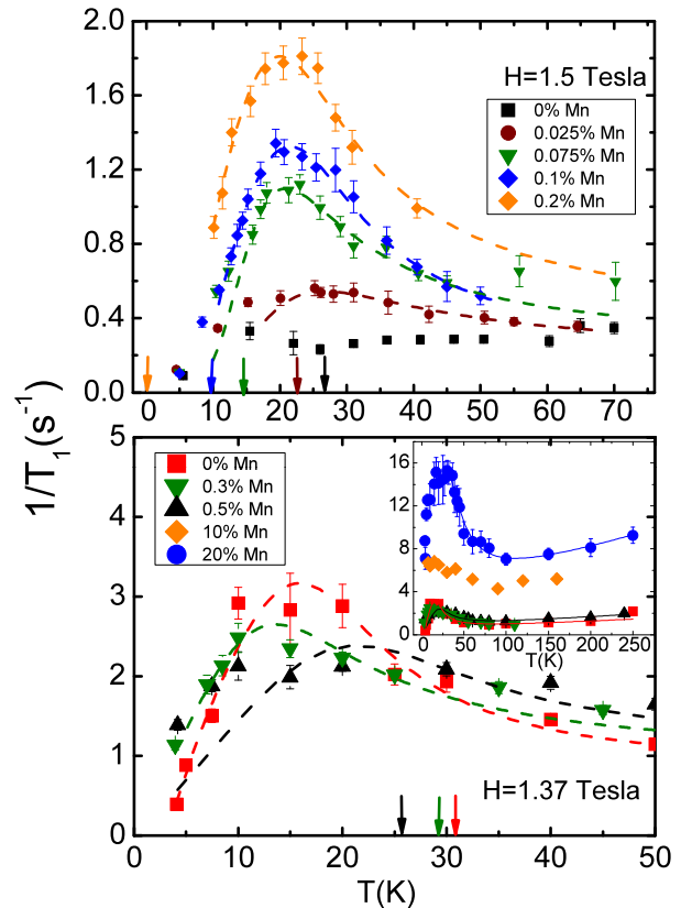
FIG. 2. (Color online) Top: Temperature dependence of ^{19}\text{F} NMR 1/T_1 for LaY0 with x up to 0.2%. Bottom: Temperature dependence of ^{19}\text{F} NMR 1/T_1 in LaY20 for Mn contents up to x = 0.5\% . In the inset the temperature ( T ) dependence is reported also for x = 10\% and x = 20\% nonsuperconducting samples. The dashed lines are fits of the data according to Eq. (3) in the text, while the arrows indicate the T_c of the different samples (decreasing with increasing x ).
