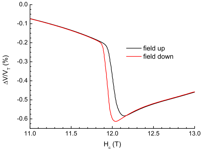
FIG. 3. (Color online) Relative velocity variation of the transverse mode showing the field hysteresis for the first-order phase transition observed at 12 T with H \parallel \hat{c} .
