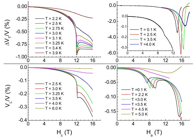
FIG. 2. (Color online) Field dependence of the relative velocity variation measured at different temperatures. On the left-hand side we present results for V_{T[100]P[010]} and V_{L[100]} with H \parallel \hat{c} , while on the right-hand side we show results obtained with H \parallel \hat{a} .
