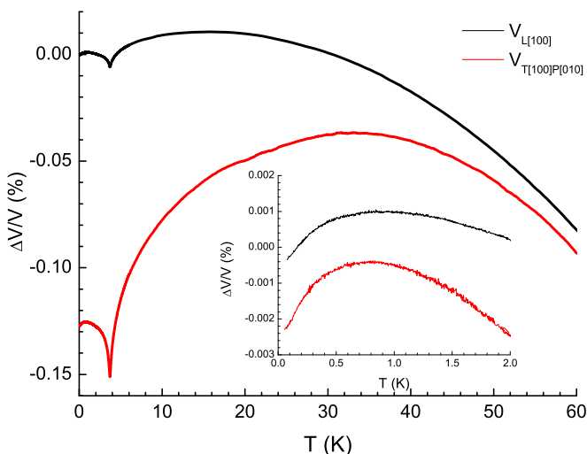
FIG. 1. (Color online) Temperature dependence (in zero field) of the relative velocity variation of the longitudinal mode V_{L[100]} (black curve) and of transverse waves polarized in the ab plane propagating along the a axis, V_{T[100]P[010]} (red curve).
