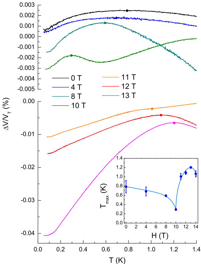
FIG. 6. (Color online) Low-temperature sound velocity measurements showing an unusual softening of the lattice at temperatures below 1 K. The round data points indicate the maximum (or inflection point for H = 11 T), T_{\max} , that we identify as the onset of the low-temperature lattice softening. The inset shows T_{\max} as a function of H \parallel \hat{a} . T_{\max} exhibits a clear cusp at around 10 T, which coincides with the field-induced phase transition from Y -type to uud order.
