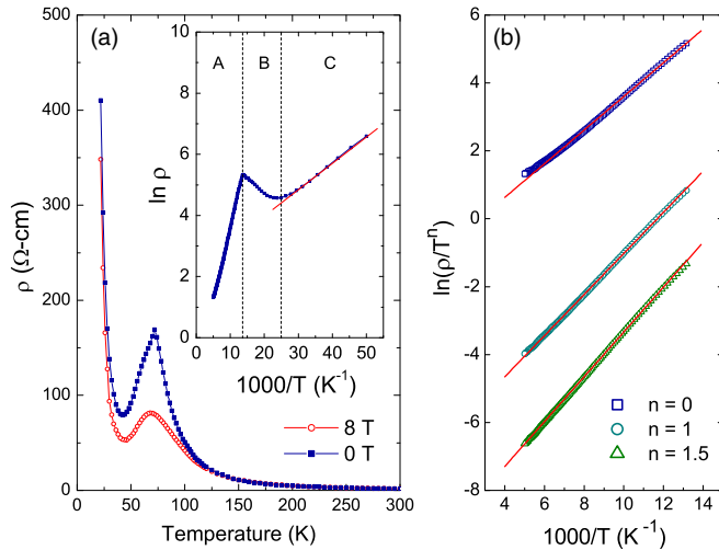
FIG. 1. (Color online) (a) Temperature dependent resistivity measured at zero field (blue) and 8 T (red). The inset indicates that the temperature dependence is consisted of two activated regions (A and C) separated by a metalliclike temperature range (B). Solid line in the inset is a fit to the simple activation law [Eq. (1)] for the low temperature resistivity. (b) The resistivity curve in a temperature range from 75 to 200 K is fitted to Eq. (1) with n = 0 for the Arrhenius activation model, n = 1 for the adiabatic small magnetic-polaron hopping model, and n = 3/2 for the nonadiabatic small magnetic-polaron hopping model.
