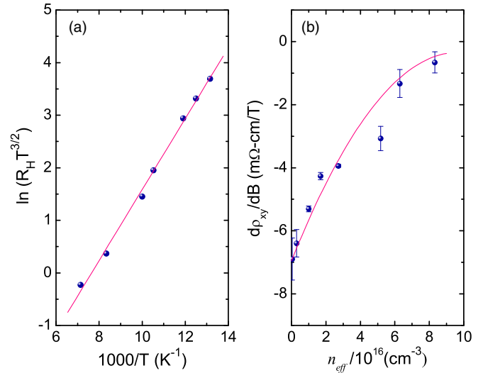
FIG. 4. (Color online) (a) The temperature dependence of the zero-field Hall coefficient of \text{Lu}_2\text{V}_2\text{O}_7 . The solid line is the best fit to the intrinsic semiconductor activation behavior [Eq. (5)]. (b) High-field Hall resistivity slope as a function of the effective carrier density calculated from the zero-field Hall coefficient at the same temperature. The solid curve is a guide to the eye. The results suggest the presence of electron donor impurities, possibly due to an oxygen deficiency.
