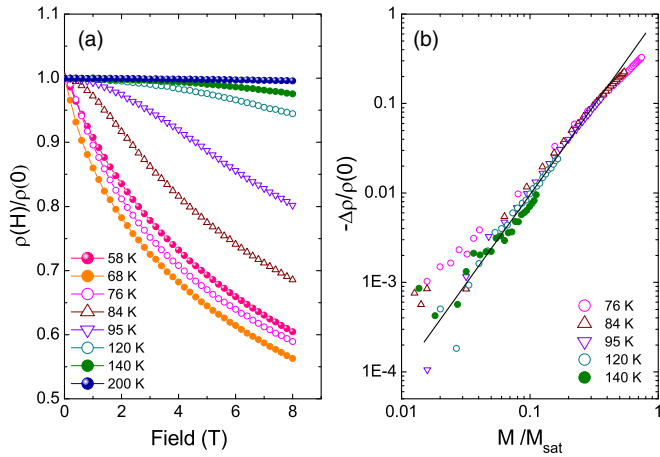
FIG. 2. (Color online) (a) The normalized resistivity of \text{Lu}_2\text{V}_2\text{O}_7 as a function of external magnetic field at selected temperatures. (b) Log-log plot of the MR versus the reduced magnetization at temperatures above T_C , which shows a power-law scaling following Eq. (2).
